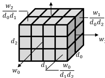
Figure 7.1: Communication model: The \text{dim\_weights}[i]=w_i express the total communication cost in the direction of dimension i . The communication cost of one process in direction i is therefore w_i / \prod_{j,j \neq i} d_j with \text{dims}[i]=d_i .
