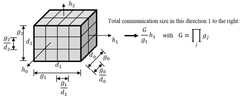
Figure 7.2: Example for the calculation of the weights. The data sizes g_i express the three dimensions of the total application data grid. The virtual process grid dimensions are expressed by d_i . The figure shows the division of the total application grid into its subdomains. The value h_i represents the halo width in a given direction when the 2-dimensional side of a subdomain is communicated to the neighbor process in that direction.
