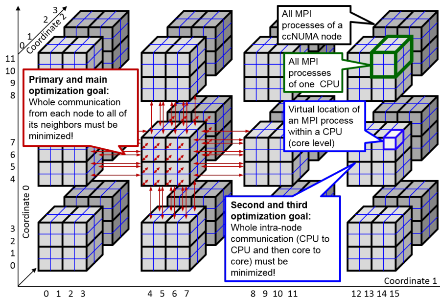
Figure 7.4: Example with 24 shared memory nodes (e.g., ccNUMA nodes), 4 NUMA-nodes (e.g., CPUs) per node and 8 MPI processes (e.g., on cores) per NUMA-node. The figure shows the 3-dimensional distribution calculated by MPI_CART_CREATE_WEIGHTED based on weight values (1/12, 1/16, 1/8).
