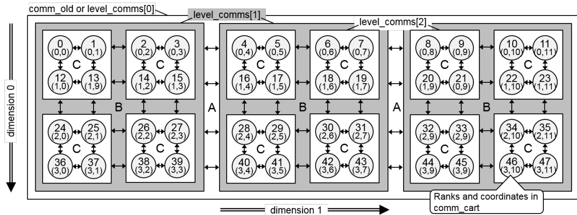
Figure 7.3: Example with a comm_old with 48 processes, ndims=2 , dim_weights=(1./4, 1./12) , and nsplit_types=2 and split_types , e.g., splitting into ccNUMA nodes and those into CPUs, and here with 4 cores per CPU and 4 CPUs per node. The level_comms[i] show this splitting of comm_old into hierarchical subcommunicators. The renumbering in comm_cart should first minimize the communication A (here, e.g., the communication between the ccNUMA nodes), then B (here, e.g., the CPU to CPU communication), and last C (here, e.g., the core to core communication)
