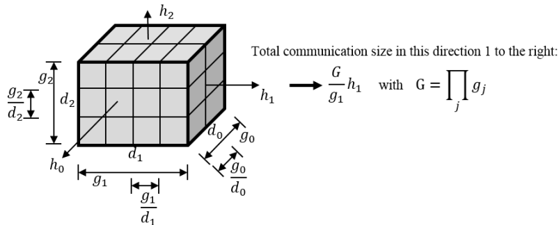
Figure 7.2: Example for the calculation of the weights. The data sizes g_i express the three dimensions of the total application data mesh. The virtual process grid dimensions are expressed by d_i . The figure shows the division of the total application mesh into its subdomains. The value h_i represents the halo width in a given direction when the 2-dimensional side of a subdomain is communicated to the neighbor process in that direction.
