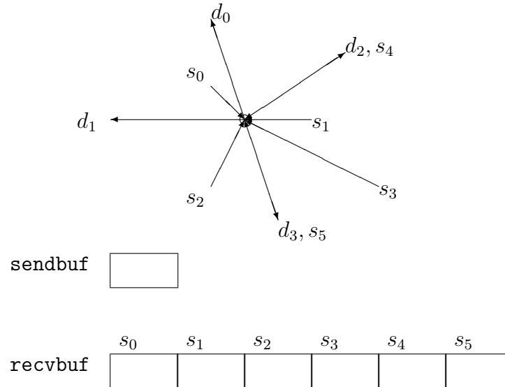
Figure 7.5: Neighborhood gather communication example.
