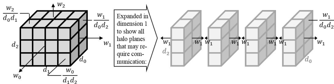
Figure 7.1: Communication model: The dim_weights[i]=w i express the total communication costs in the direction of dimension i , i.e., accumulated over all MPI processes that are part of the same surface in this direction. The figure to the right shows all communications in the positive and negative direction of dimension 1. The communication costs of one process in direction i is therefore w_i / \prod_{j,j \neq i} d_j with dims[i]=d i , which are returned from this procedure.
