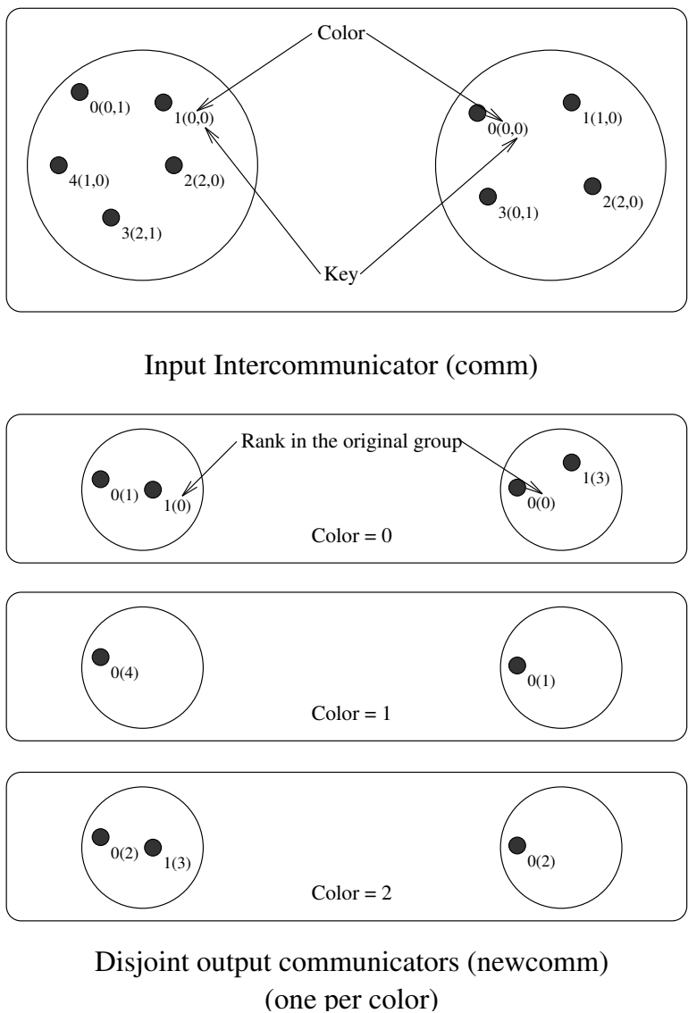
43 Figure 6.2: Intercommunicator construction achieved by splitting an existing intercommuni- 44 cator with MPI_COMM_SPLIT extended to intercommunicators.
