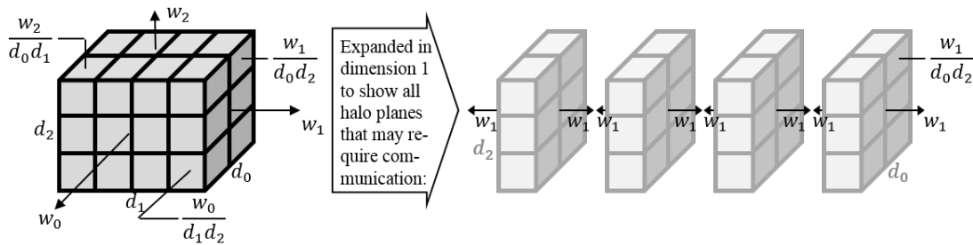
Figure 7.4: Communication model: w_i should express the accumulated communication size in the direction of dimension i , i.e., accumulated over all MPI processes that are part of the same surface in this direction. The figure to the right shows all communications in the positive and negative direction of dimension 1. The communication size of one process in direction i is therefore w_i / \prod_{j,j \neq i} d_j .
