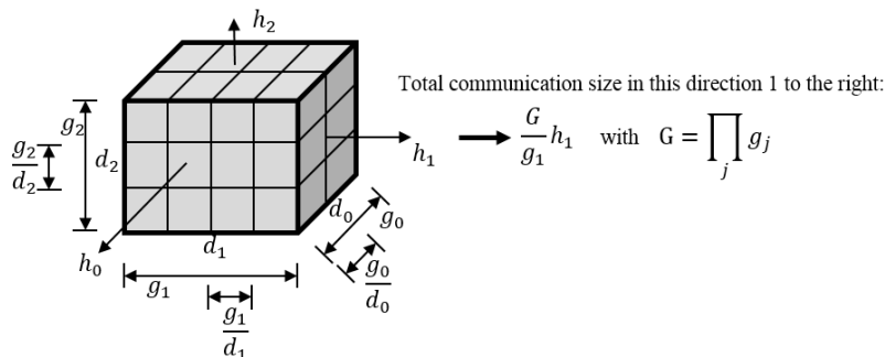
Figure 7.3: Example for the calculation of the accumulated communication size in each dimension. The data sizes g_i express the three dimensions of the total application data mesh. The virtual process grid dimensions are expressed by d_i . The figure shows the division of the total application mesh into its subdomains. The value h_i represents the halo width in a given direction when the 2-dimensional side of a subdomain is communicated to the neighbor process in that direction.
