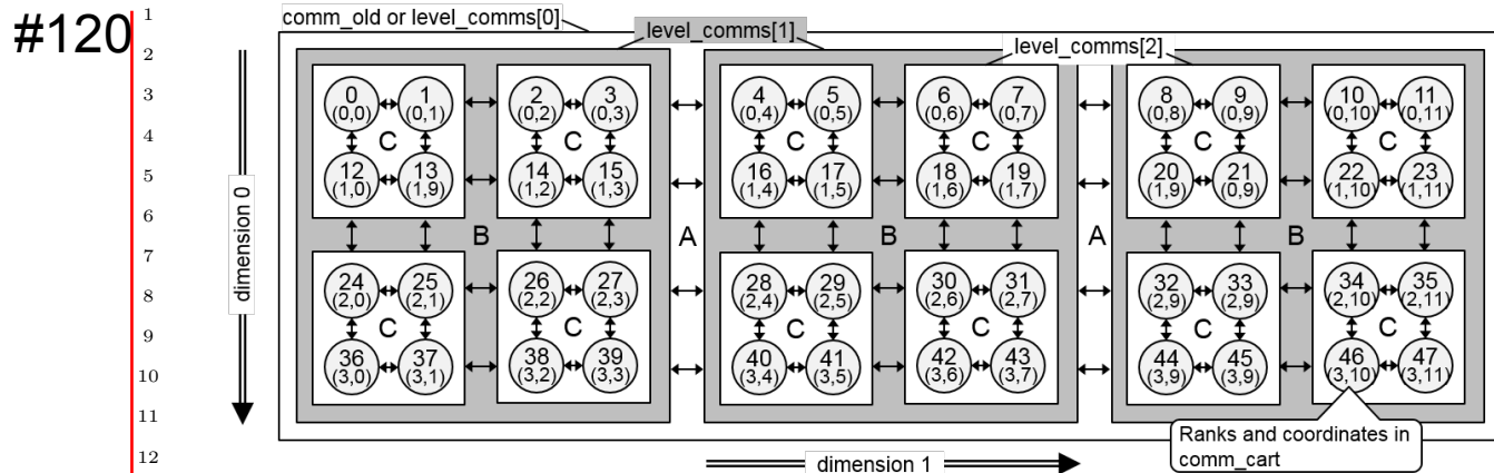
Figure 7.1: Example with a comm_old with 48 processes, ndims=2 , dim_weights=(1./4, 1./12) , and nsplit_types=2 and split_types , e.g., splitting into ccNUMA nodes and those into CPUs, and here with 4 cores per CPU and 4 CPUs per node. The level_comms[i] show this splitting of comm_old into hierarchical subcommunicators. The renumbering in comm_cart should first minimize the communication A (here, e.g., the communication between the ccNUMA nodes), then B (here, e.g., the CPU to CPU communication), and last C (here, e.g., the core to core communication)
