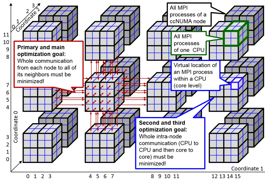
Figure 7.2: Example with 24 shared memory nodes (e.g., ccNUMA nodes), 4 NUMA-nodes (e.g., CPUs) per node and 8 MPI processes (e.g., on cores) per NUMA-node. The figure shows the 3-dimensional distribution calculated by MPI_CART_CREATE_WEIGHTED based on weight values (1/12, 1/16, 1/8).
