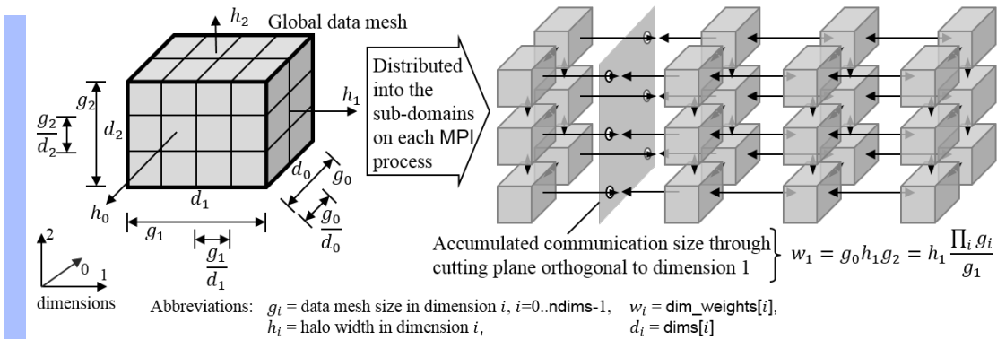
Figure 7.2: Example for the calculation of the accumulated communication size w_{i,i=0..2} in each dimension. The data mesh sizes g_{i,i=0..2} express the three dimensions of the total application data mesh. The value h_i represents the halo width in a given direction when the 2-dimensional side of a subdomain is communicated to the neighbor process in that direction. The values w_{i,i=0..2} are used as input argument dim_weights[i] in MPI_DIMS_CREATE_WEIGHTED or MPI_CART_CREATE_WEIGHTED , which return an optimized factorization of the number of processes into the dimensions of the virtual process grid, expressed by d_i . The figure shows the resulting division of the total application mesh into its subdomains.
