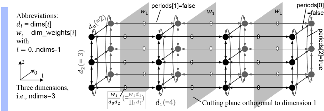
Figure 7.1: Example of a virtual process grid with 3 dimensions and 24 MPI processes. The arguments \text{dim\_weights}[i]_{i=0.. \text{ndims}-1} , abbreviated with w_i , should be specified as the accumulated message size (in bytes) communicated in one communication step through each cutting plane orthogonal to dimension d_i and in each of the two direction. Based on the factorization of the number of processes into the d_i , the expected size of each message along the edges of the virtual process grid will be w_i / \prod_{j \neq i} d_j .
