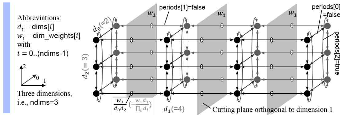
Figure 7.1: Example of a virtual process grid with 3 dimensions and 24 MPI processes. The arguments \text{dim\_weights}[i]_{i=0..(\text{ndims}-1)} , abbreviated with w_i , should be specified as the accumulated message size (in bytes) communicated in one communication step through each cutting plane orthogonal to dimension d_i and in each of the two directions. Based on the factorization of the number of processes into the d_i , the expected size of each message along the edges of the virtual process grid will be w_i / \prod_{j \neq i} d_j .
