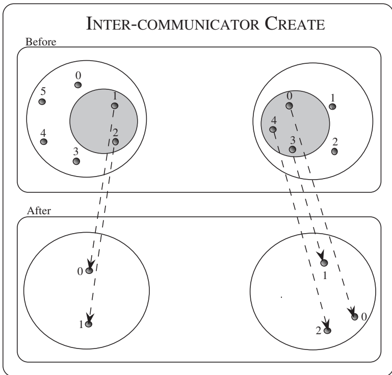
41 Figure 6.1: Intercommunicator creation using MPI_COMM_CREATE extended to intercom- 42 municators. The input groups are those in the grey circle. 43
