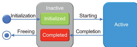
Figure 2.3: State Transition Diagram for Persistent Operations
