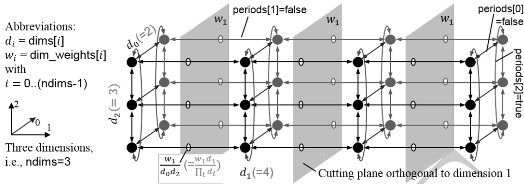
Figure 7.1: Example of a virtual process grid with 3 dimensions and 24 MPI processes. The arguments dim_weights[i] i =0.. (ndims-1) , abbreviated with w_i , should be specified as the accumulated message size (in bytes) communicated in one communication step through each cutting plane orthogonal to dimension d_i and in each of the two directions. Based on the factorization of the number of processes into the d_i , the expected size of each message along the edges of the virtual process grid will be w_i / \prod_{j \neq i} d_j .
