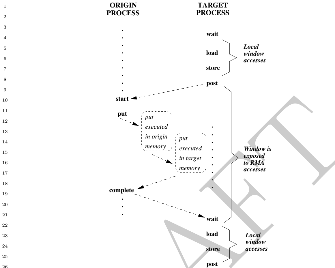
Figure 11.2: Active target communication. Dashed arrows represent synchronizations (ordering of events).
