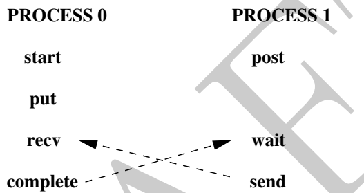
Figure 11.7: Deadlock situation
