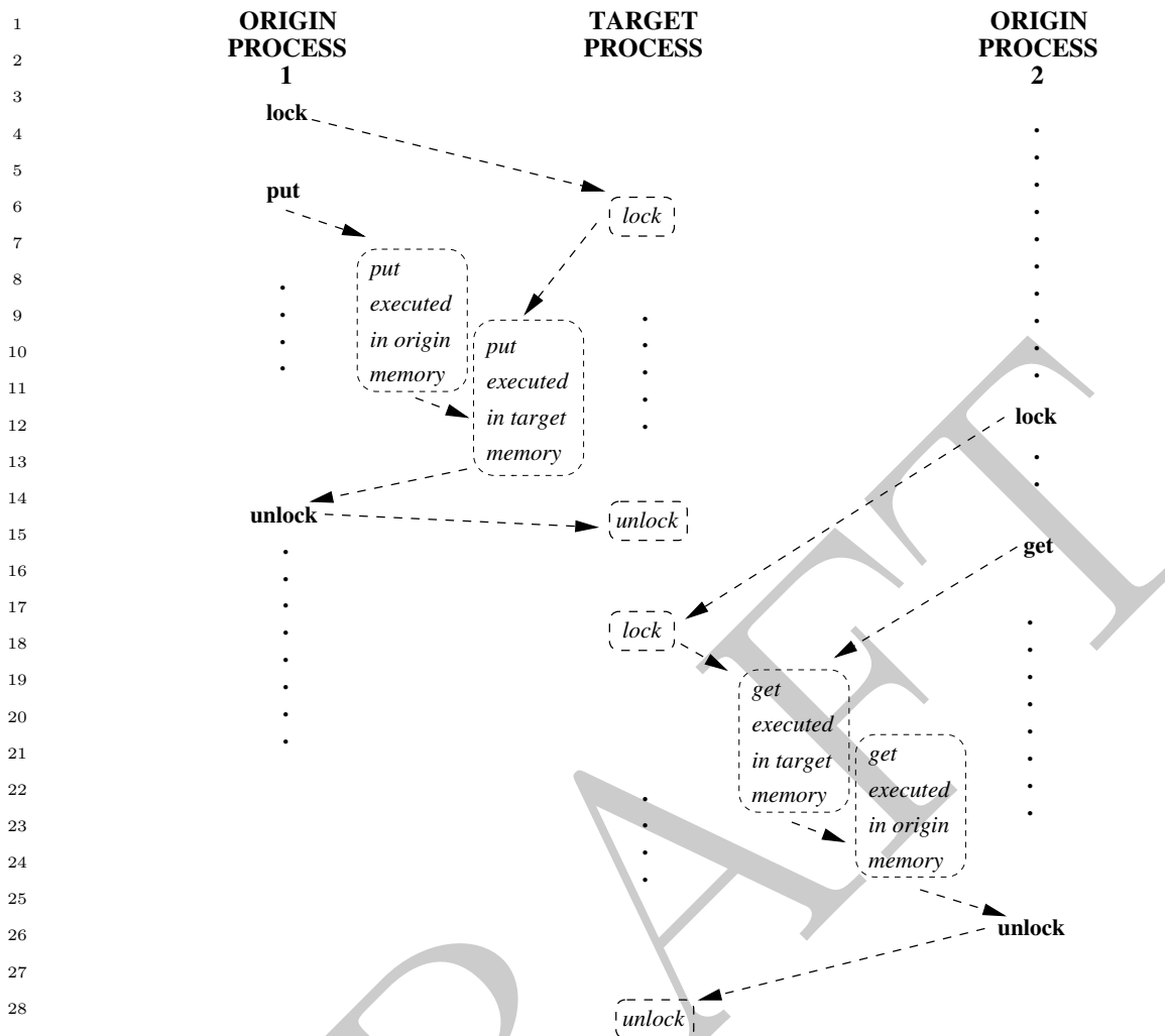
Figure 11.4: Passive target communication. Dashed arrows represent synchronizations (ordering of events).
