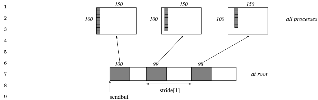
11 Figure 6.11: The root scatters blocks of 100-i ints into column i of a 100 \times 150 C array. 12 At the sending side, the blocks are \text{stride}[i] ints apart.
