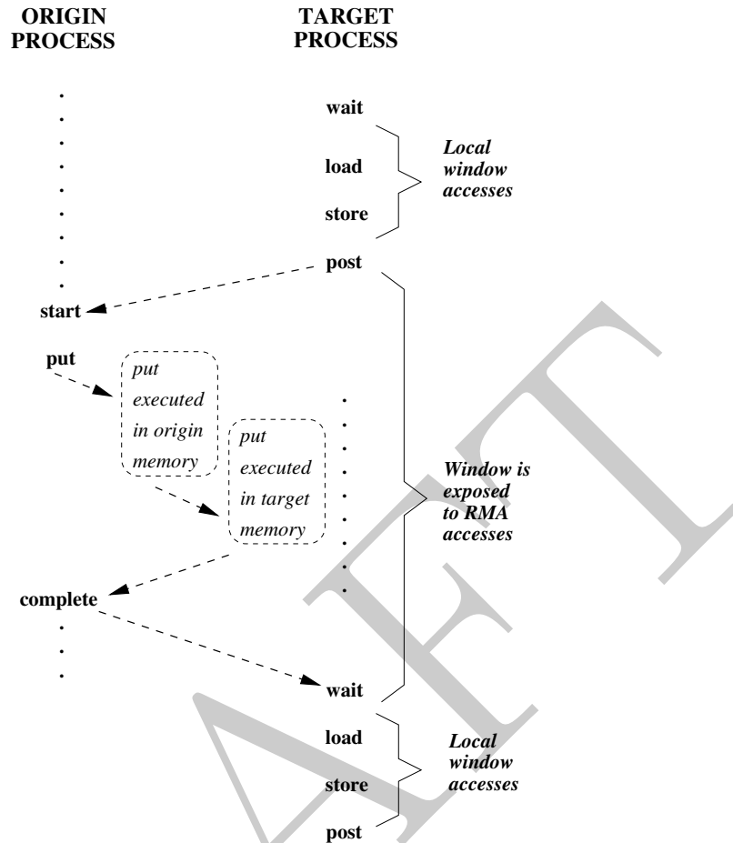
Figure 12.2: Active target communication. Dashed arrows represent synchronizations (ordering of events).
