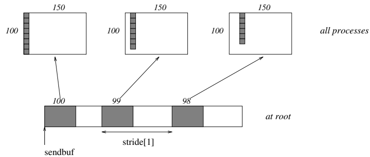
Figure 6.11: The root scatters blocks of 100-i ints into column i of a 100 \times 150 C array. At the sending side, the blocks are \text{stride}[i] ints apart.
