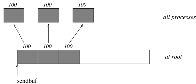
Figure 6.9: The root MPI process scatters sets of 100 ints to each MPI process in the group.
