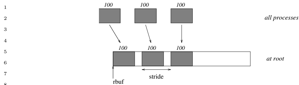
Figure 6.5: The root MPI process gathers 100 ints from each MPI process in the group, each set is placed stride ints apart.
