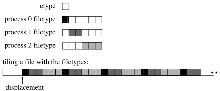
Figure 14.2: Partitioning a file among parallel MPI processes
