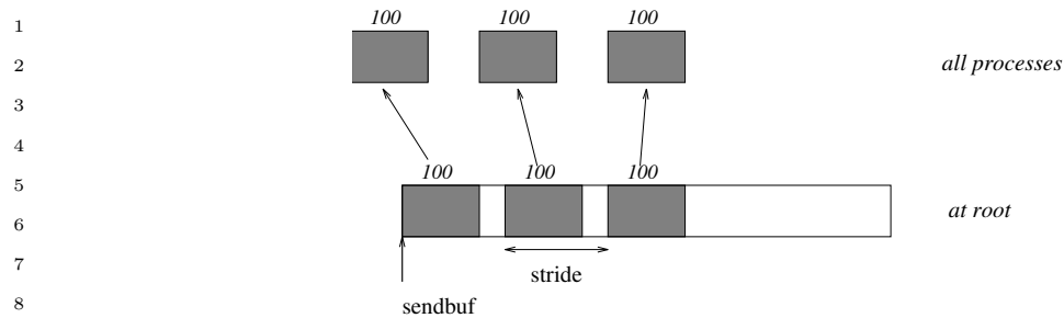
Figure 6.10: The root MPI process scatters sets of 100 ints, moving by stride ints from send to send in the scatter.
