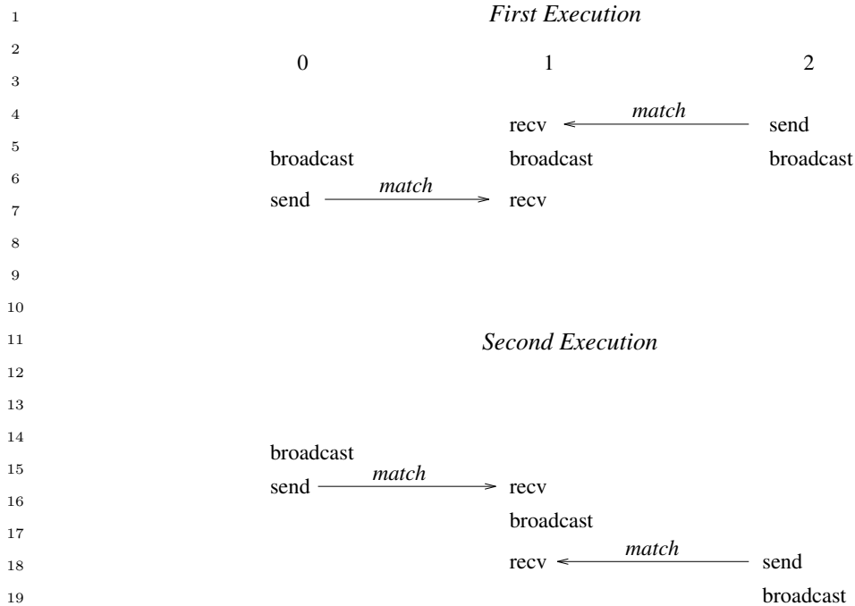
24 25 26 27 28 29 30 31 32 33 Figure 6.12: A race condition causes nondeterministic matching of sends and receives. One cannot rely on synchronization from a broadcast to make the program deterministic.
