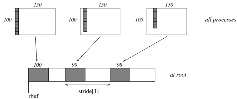
Figure 6.8: The root process (ranked with respect to the referenced communicator) gathers 100-i ints from column i of a 100 \times 150 C array, and each set is placed \text{stride}[i] ints apart (a varying stride).
