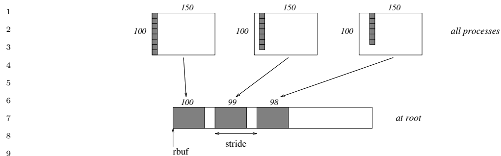
Figure 6.7: The root MPI process (ranked with respect to the group of the communicator) gathers 100-i ints from column i of a 100 \times 150 C array, and each set is placed stride ints apart.
