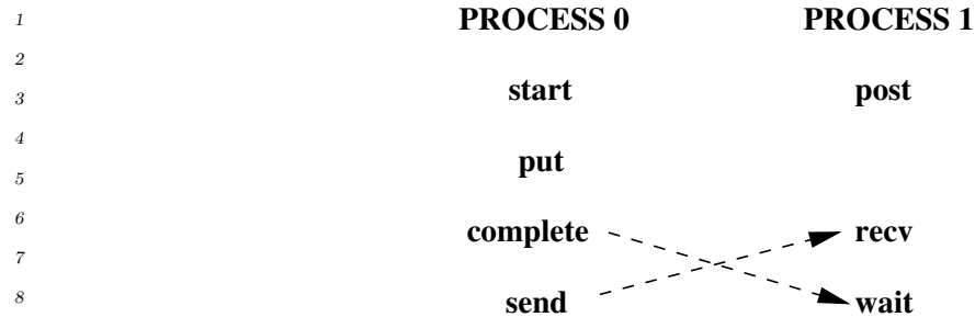
Figure 12.8: No deadlock
