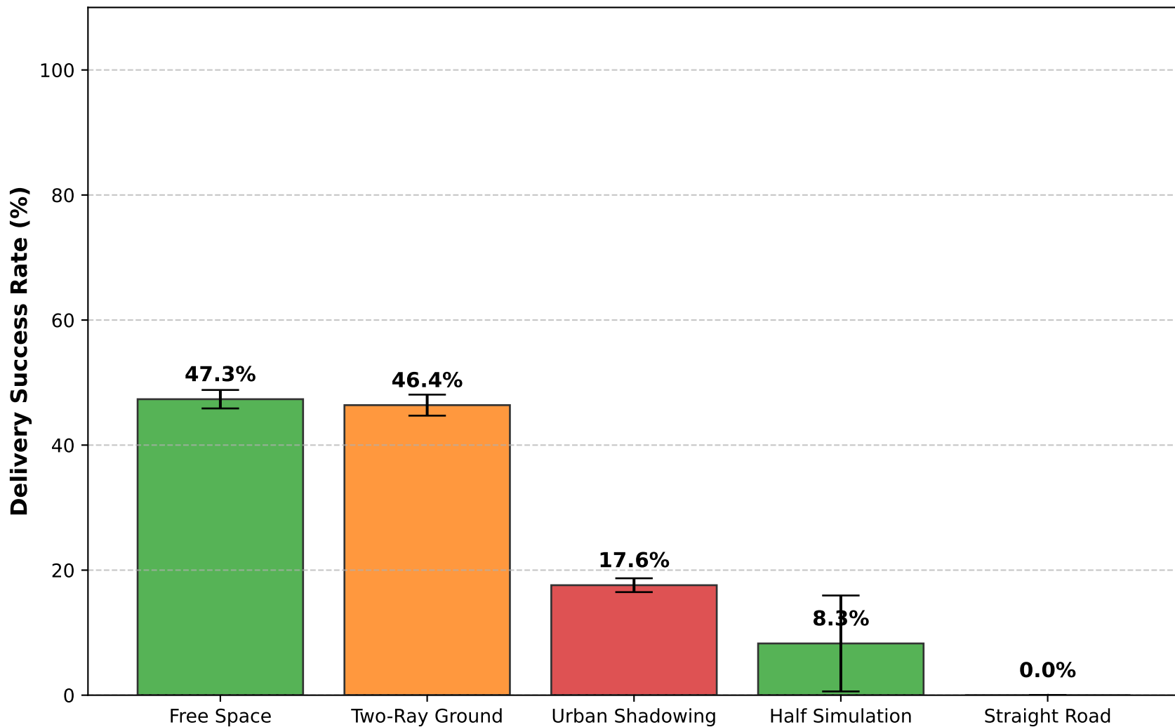
V2V Packet Delivery Ratio (PDR) with 95% CI
