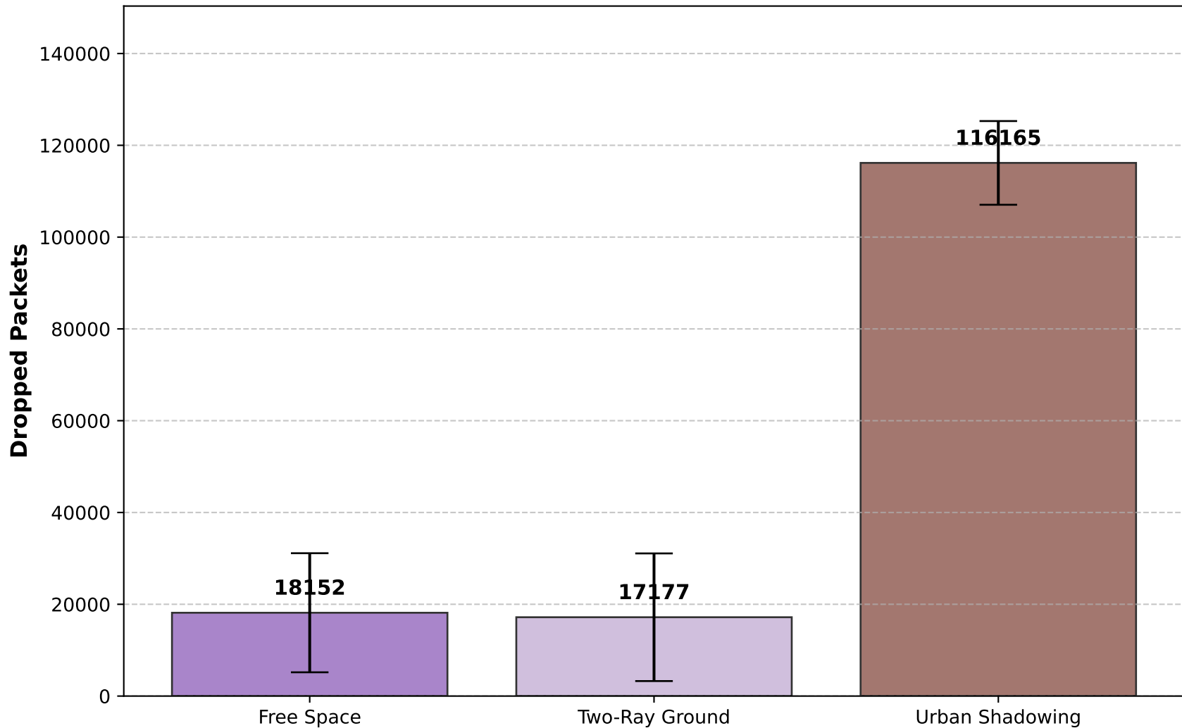
Packets Dropped due to Interference with 95% CI
