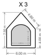
Window 窗户
