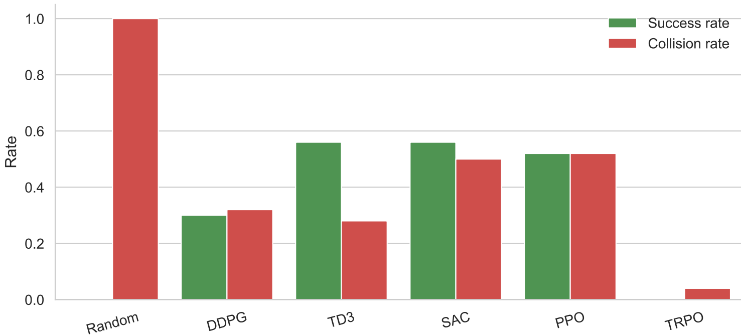
Success and collision rates
