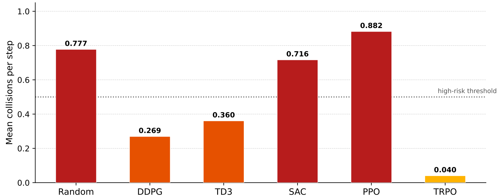
Collision intensity per agent (mean collisions per step)
