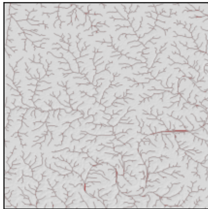
(c) channel network at matched NHD density
