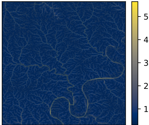
(b) D8 flow accumulation (log scale)
