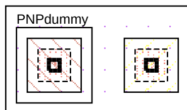
Substrate PNP
