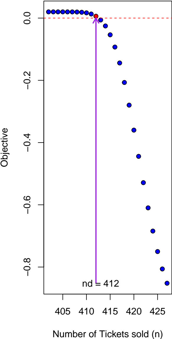
Discrete Solution (N=400, g=0.02, p=0)rmal Approximation (N=400, g=0.02, p
