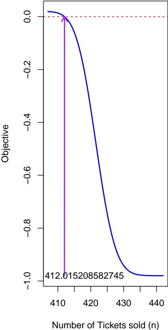
Discrete Solution (N=400, g=0.02, p=0)rmal Approximation (N=400, g=0.02, p
