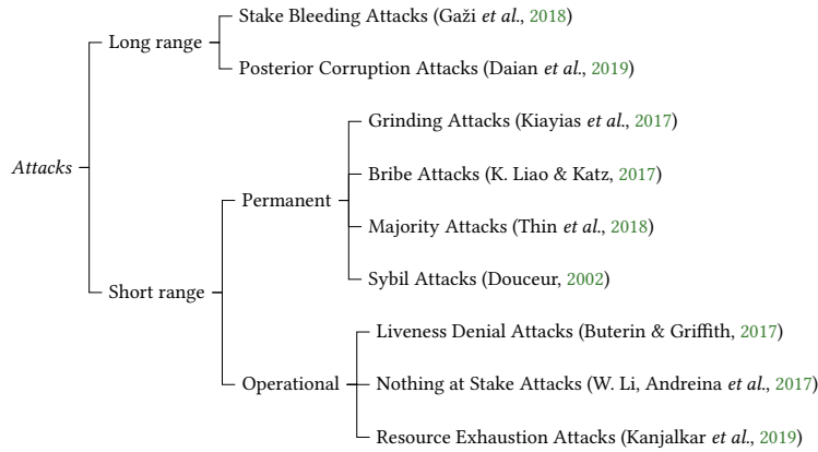
Figure 7.1: Categorisation of attacks on IdAPoS systems.
