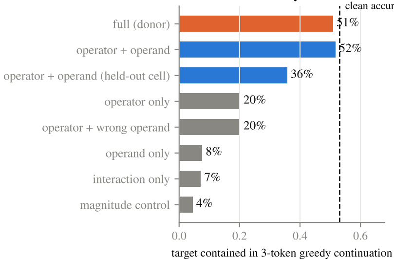
Behavioral sufficiency: does the model SAY it?
