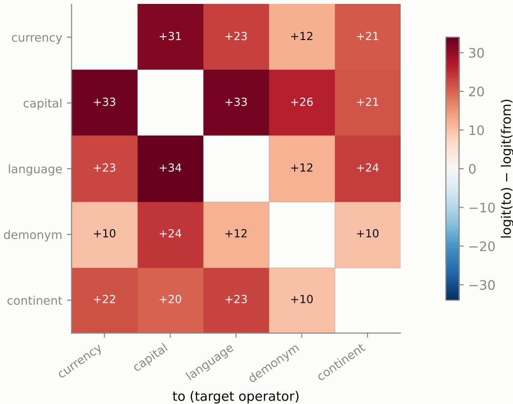
Inject v(\text{to}) - v(\text{from}) — “to” wins
