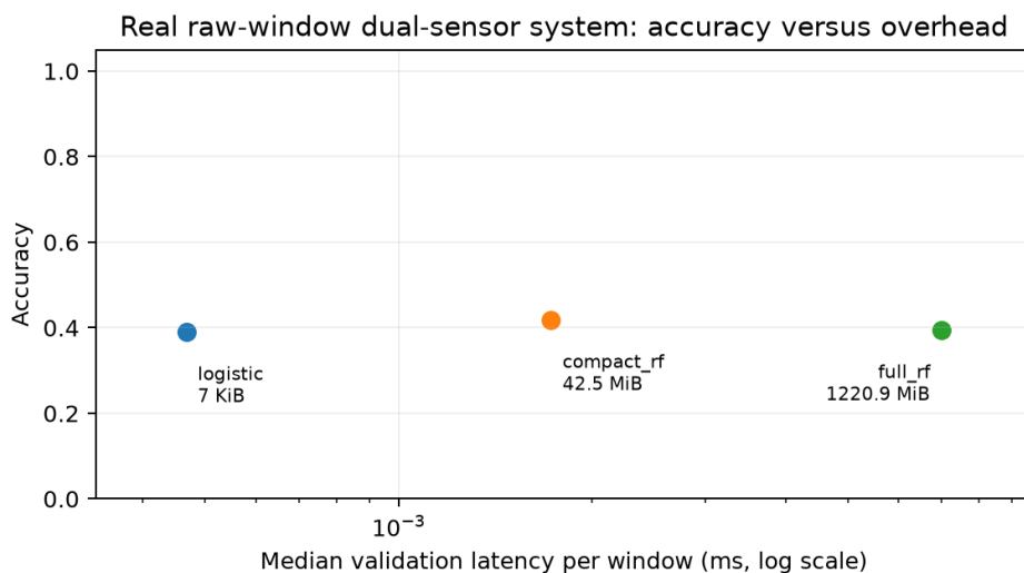
Figure 5. User-disjoint validation accuracy versus per-window prediction latency. Labels report serialized estimator size; latency excludes feature extraction.
