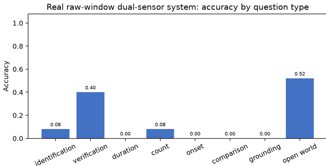
Figure 2. Exact-match accuracy on 75 held-out real-data questions per type.
