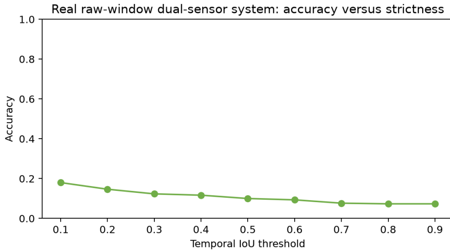
Figure 4. Grounded temporal accuracy as the required interval IoU increases from 0.1 to 0.9.
