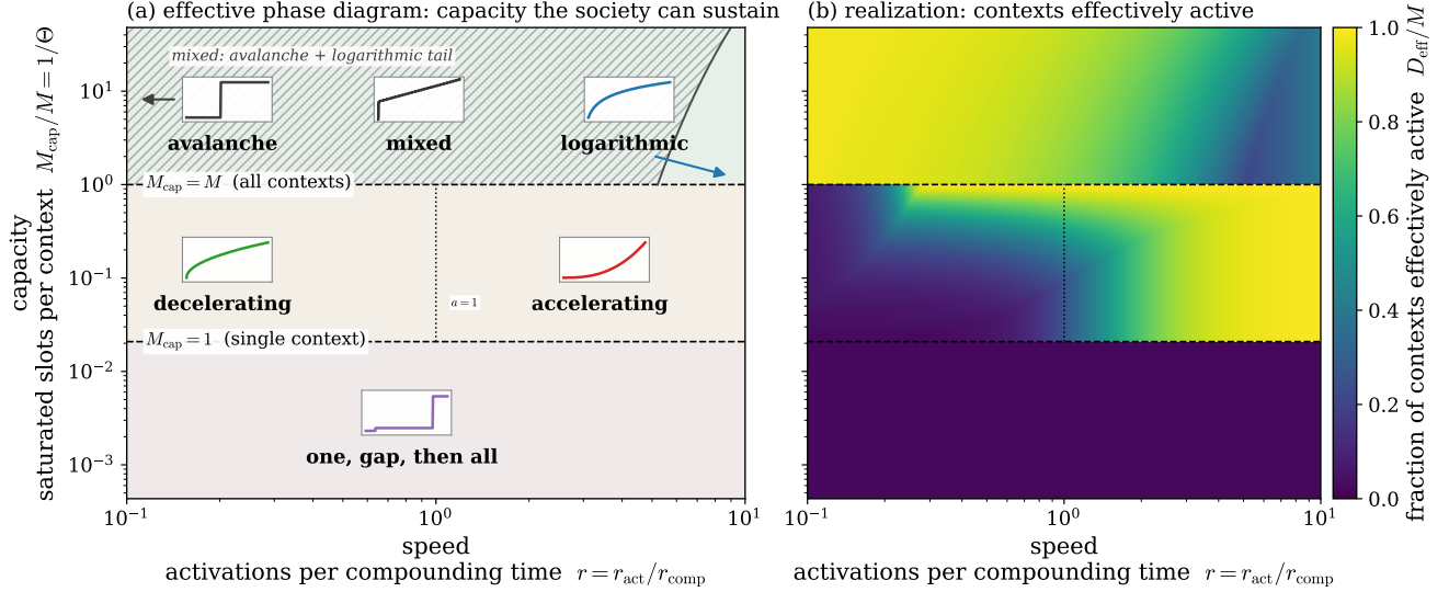
FIG. 3. Cascade types and repertoire size over replicator dynamics. Endogenous cascade regimes over the two coordinates that separate them. The horizontal axis ( speed ) is r = r_{\text{act}}/r_{\text{comp}} , the number of axes that activate per compounding time 1/r_{\text{comp}} , fixed by the dispersion of the seeded repertoire through Eq. (26). The vertical axis ( capacity ) is M_{\text{cap}}/M , the saturated slots per context, that is the fraction of the M candidate schemas the finite social capacity can sustain as live contexts ( M_{\text{cap}} = U_{\text{cap}}/u_{\text{cap}} ). (a) Capacity: the contexts the society can sustain, a stationary-state property fixed by \Theta = M/M_{\text{cap}} alone, which splits the plane into three bands with sharp counting-threshold boundaries: all M contexts, a graded cluster of M_{\text{cap}} , or one. Inset sketches show the sequence of activations the transient sort passes through, set by r : avalanche to logarithmic in the thick band ( \Theta \leq 1 ), decelerating ( a > 1 ) to accelerating ( a < 1 ) across a = 1 in the middle band, and one onset, a gap, then all the rest in the thin band. The left-hand arrow marks r \rightarrow 0 , where the cascade is a pure avalanche. The random Marčenko–Pastur class (iv of Fig. 2) is absent because it is an unorganized initial condition rather than an endpoint the loop selects (Sec. IV B). Within the thick band a saturated cluster coexists with a geometric tail (hatched) below the exact boundary r = M/L(\Theta) . The right-hand arrow runs from the logarithmic sketch past that boundary to a purely geometric spectrum, and the inset shows N(\beta) at a coexistence point—an early jump as the cluster ignites at once, then the tail’s gradual rise. (b) Realization: the contexts effectively active , the participation ratio D_{\text{eff}} = (\sum_k \mu_k)^2 / \sum_k \mu_k^2 of the spectrum \{\mu_k = u_k\} , normalized by M . It depends on how far the transient sort has progressed, hence on r , and falls below capacity wherever the sort is incomplete—bright on the accelerating side, darker on the decelerating side. The difference between the panels measures distance from the stationary endpoint. Exact boundaries, their mean-field status, the ceiling u_{\text{cap}} , and the held-fixed groups ( \alpha\langle\lambda\rangle/\kappa , \beta\mu_1/\gamma , M/d ) in Sec. IV B.
