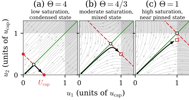
FIG. 4. The pinning saddle across \Theta . Phase portraits of the two-schema strength dynamics Eq. (24) in (u_1, u_2) , units of u_{\text{cap}} , at three budgets U_{\text{cap}} = Mu_{\text{cap}}/\Theta ( M = 2 throughout): the pinned (saddle) point (black-edged circle), at U_{\text{cap}}/2 , moves out along the stable manifold u_1 = u_2 (green) panel to panel as U_{\text{cap}} \rightarrow Mu_{\text{cap}} . The black curve is a trajectory from one seeded start (black dot, the same in all three panels), which grows along the stable manifold and then departs along the unstable one. (a) \Theta = 4 : the budget alone halts growth well inside u_{\text{cap}} , so the unstable manifold (red, condensation) runs to a genuinely reached bare condensate (filled circles). (b) \Theta = 4/3 : the ceiling is now reached first, arresting the same departure at u_{\text{cap}} (red square) before it reaches the excluded region u_1 > u_{\text{cap}} or u_2 > u_{\text{cap}} (shaded). (c) \Theta = 1 : capacity exactly meets demand ( M_{\text{cap}} = M ), so the saddle sits at u_1 = u_2 = u_{\text{cap}} and the trajectory is arrested (red square) just short of it. Panel sub-titles name the resulting state.
