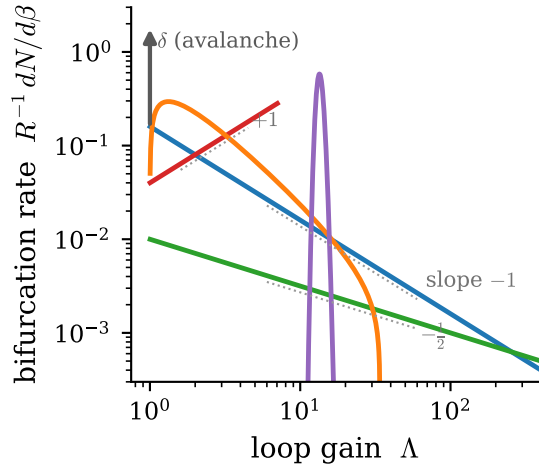
(b) bifurcation rate
