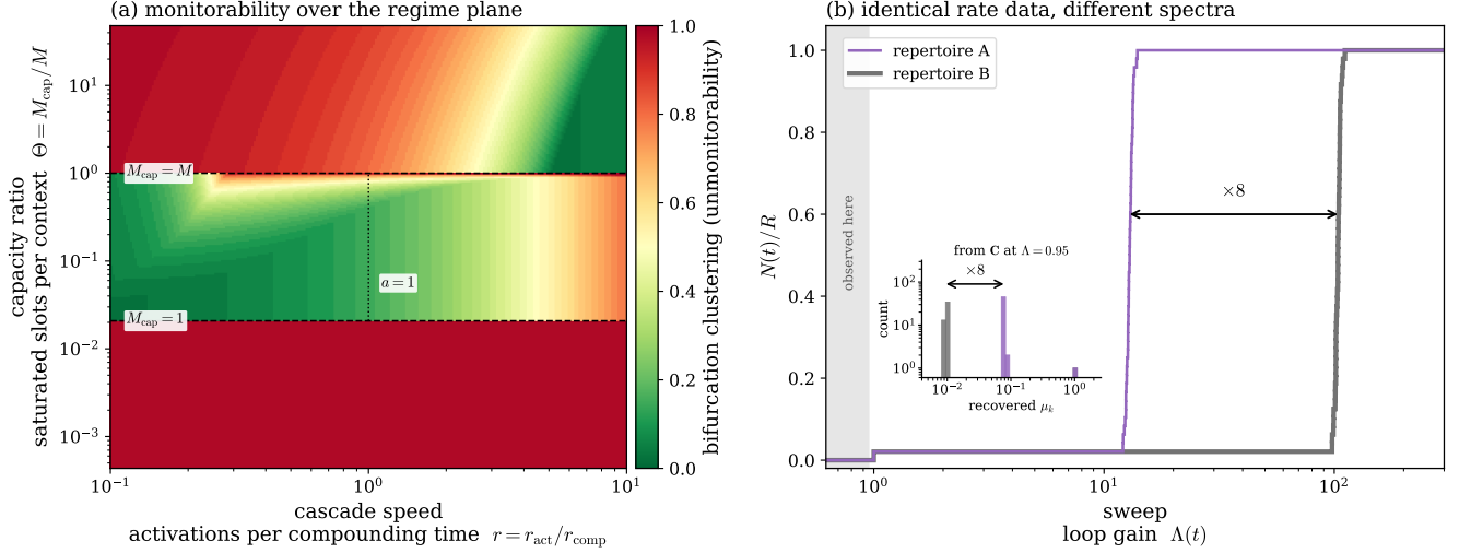
FIG. 5. Monitoring the cascade. (a) Monitorability over the (\Theta, r) plane: the clustering of bifurcation onsets (colour; the maximal share arriving within \Delta \ln \Lambda = 0.15 , hence unmonitorability), red where onsets cluster into a single burst (avalanche, spiked) and green where they resolve into a sequence (logarithmic, decelerating). The \Theta boundaries are sharp, the r dependence a smooth crossover. Regime layout as in Fig. 4. (b) The measurement term, under a linear sweep of the loop gain \Lambda(t) . Two repertoires whose counting functions coincide over the whole plotted range: each activates one axis at \Lambda = 1 and then stays quiescent. In repertoire A the remaining R - 1 modes sit just below threshold and avalanche at \Lambda = 13 ; in repertoire B the same modes sit far below and do not activate until \Lambda = 104 . The two spectra differ only below 1/\Lambda , which the bifurcation rate never samples, so rate extrapolation cannot separate them. Inset: the gain spectrum recovered from the subcritical covariance \mathbf{C} = \frac{\sigma_\omega^2}{2\gamma} (\mathbf{I}_{d \times d} - \mathbf{\Lambda})^{-1} at \Lambda = 0.95 , before either has bifurcated. The two recovered bulks are separated by the same factor of 8 that separates the two rises, since an onset sits at 1/\mu . The paired arrows mark it. The inversion amplifies a 7% difference in covariance eigenvalues into that factor, so the number of agents sampled sets the practical limit (Sec. V).
