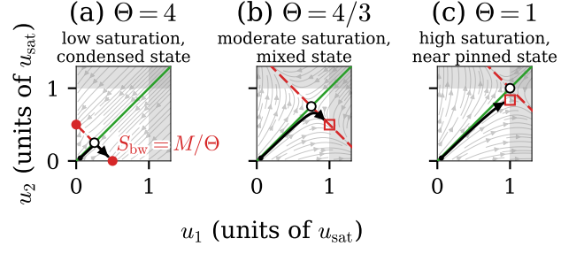
FIG. 4. The pinning saddle across \Theta . Phase portraits of the two-schema strength dynamics Eq. (22) in (u_1, u_2) , units of u_{\text{sat}} , at three budgets S_{bw} ( M = 2 throughout): the pinned (saddle) point (black-edged circle), at S_{bw}/2 , moves out along the stable manifold u_1 = u_2 (green) panel to panel as S_{bw} \rightarrow Mu_{\text{sat}} . The black curve is a trajectory from one seeded start (black dot, the same in all three panels), which grows along the stable manifold and then departs along the unstable one. (a) \Theta = 4 : the budget alone halts growth well inside u_{\text{sat}} , so the unstable manifold (red, condensation) runs to a genuinely reached bare condensate (filled circles). (b) \Theta = 4/3 : the ceiling is now reached first, arresting the same departure at u_{\text{sat}} (red square) before it reaches the excluded region u_1 > u_{\text{sat}} or u_2 > u_{\text{sat}} (shaded). (c) \Theta = 1 : capacity exactly meets demand ( M_{\text{cap}} = M ), so the saddle sits at u_1 = u_2 = u_{\text{sat}} and the trajectory is arrested (red square) just short of it. Panel sub-titles name the resulting state.
