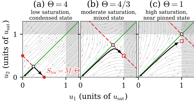
FIG. 4. The pinning saddle across \Theta . Phase portraits of the two-schema strength dynamics Eq. (22) in (u_1, u_2) , units of u_{\text{sat}} , at three budgets S_{\text{bw}} ( M = 2 throughout): the pinned (saddle) point (black-edged circle), at S_{\text{bw}}/2 , moves out along the stable manifold u_1 = u_2 (green) panel to panel as S_{\text{bw}} \rightarrow Mu_{\text{sat}} . The black curve is a trajectory from one seeded start (black dot, the same in all three panels), which grows along the stable manifold and then departs along the unstable one. (a) \Theta = 4 : the budget alone halts growth well inside u_{\text{sat}} , so the unstable manifold (red, condensation) runs to a genuinely reached bare condensate (filled circles). (b) \Theta = 4/3 : the ceiling is now reached first, arresting the same departure at u_{\text{sat}} (red square) before it reaches the excluded region u_1 > u_{\text{sat}} or u_2 > u_{\text{sat}} (shaded). (c) \Theta = 1 : capacity exactly meets demand ( M_{\text{cap}} = M ), so the saddle sits at u_1 = u_2 = u_{\text{sat}} and the trajectory is arrested (red square) just short of it. Panel sub-titles name the resulting state.
