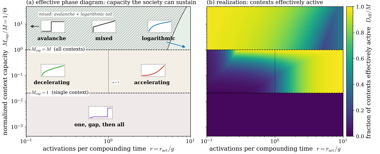
FIG. 3. Cascade types and thickness over replicator dynamics. Endogenous cascade regimes over the two coordinates that separate them— r = r_{\text{act}}/g , the number of axes that activate per compounding time (horizontal), fixed by the dispersion of the seeded repertoire through Eq. (26), and normalized context capacity M_{\text{cap}}/M (vertical), the fraction of the M candidate schemas the finite social bandwidth can sustain as live contexts ( M_{\text{cap}} = S_{\text{bw}}/u_{\text{sat}} ). (a) Capacity: the contexts the society can sustain, a stationary-state property fixed by \Theta = M/M_{\text{cap}} alone, which splits the plane into three bands with sharp counting-threshold boundaries: all M contexts, a graded cluster of M_{\text{cap}} , or one. Glyphs sketch the cascade N(\beta) the transient sort passes through en route, set by r : avalanche to logarithmic in the thick band, decelerating ( a > 1 ) to accelerating ( a < 1 ) across a = 1 in the middle band, and one onset, a gap, then all the rest in the thin band. The left-hand arrow marks r \rightarrow 0 , where the cascade is a pure avalanche. The random Marčenko–Pastur class (iv of Fig. 2) is absent because it is an unorganized initial condition rather than an endpoint the loop selects (Sec. VC). Within the thick band a saturated cluster coexists with a geometric tail (hatched) below the exact boundary r = M/L(\Theta) . The right-hand arrow runs from the logarithmic glyph past that boundary to a purely geometric spectrum, and the inset shows N(\beta) at a coexistence point—an early jump as the cluster ignites at once, then the tail’s gradual ramp. (b) Realization: the contexts effectively active, the participation ratio D_{\text{eff}} = (\sum_k \mu_k)^2 / \sum_k \mu_k^2 of the gain spectrum \{\mu_k = 2\pi'(0)u_k\} , normalized by M . It depends on how far the transient sort has progressed, hence on r , and falls below capacity wherever the sort is incomplete—bright on the accelerating side, darker on the decelerating side. The difference between the panels measures distance from the stationary endpoint. Exact boundaries, their mean-field status, the ceiling u_{\text{sat}} , and the held-fixed groups (\alpha(\lambda)/\kappa, \beta\mu_1/\gamma, M/d) in Sec. VC.
