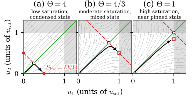
FIG. 4. The pinning saddle across \Theta . Phase portraits of the two-schema strength dynamics Eq. (22) in (u_1, u_2) , units of u_{\text{sat}} , at three budgets S_{\text{bw}} ( M = 2 throughout): the pinned (saddle) point (black-edged circle), at S_{\text{bw}}/2 , moves out along the stable manifold u_1 = u_2 (green) panel to panel as S_{\text{bw}} \rightarrow Mu_{\text{sat}} . The black curve is a trajectory from one seeded start (black dot, the same in all three panels), which grows along the stable manifold and then departs along the unstable one. (a) \Theta = 4 : the budget alone halts growth well inside u_{\text{sat}} , so the unstable manifold (red, condensation) runs to a genuinely reached bare condensate (filled circles). (b) \Theta = 4/3 : the ceiling is now reached first, arresting the same departure at u_{\text{sat}} (red square) before it reaches the excluded region u_1 > u_{\text{sat}} or u_2 > u_{\text{sat}} (shaded). (c) \Theta = 1 : capacity exactly meets demand ( M_{\text{cap}} = M ), so the saddle sits at u_1 = u_2 = u_{\text{sat}} and the trajectory is arrested (red square) just short of it. Panel sub-titles name the resulting state.
