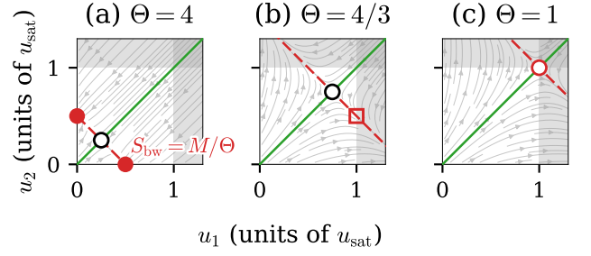
FIG. 4. The pinning saddle across \Theta . Phase portraits of the two-schema strength dynamics Eq. (22) in (u_1, u_2) , units of u_{\text{sat}} , at three budgets S_{\text{bw}} ( M = 2 throughout): the pinned (saddle) point (black-edged circle), at S_{\text{bw}}/2 , climbs the stable manifold u_1 = u_2 (green) panel to panel as S_{\text{bw}} \rightarrow M u_{\text{sat}} . (a) \Theta = 4 : the budget alone halts growth well inside u_{\text{sat}} , so the unstable manifold (red, condensation) runs to a genuinely reached bare condensate (filled circles). (b) \Theta = 4/3 : the ceiling is now reached first, arresting the same flight at u_{\text{sat}} (red square) before it reaches the excluded region u_1 > u_{\text{sat}} or u_2 > u_{\text{sat}} (shaded). (c) \Theta = 1 : the saddle itself (now red-edged) sits exactly at u_1 = u_2 = u_{\text{sat}} , the boundary where capacity exactly meets demand ( M_{\text{cap}} = M ).
