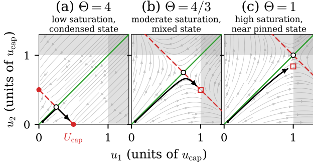
FIG. 4. The pinning saddle across \Theta . Phase portraits of the two-schema strength dynamics Eq. (22) in (u_1, u_2) , units of u_{\text{cap}} , at three budgets U_{\text{cap}} = Mu_{\text{cap}}/\Theta ( M = 2 throughout): the pinned (saddle) point (black-edged circle), at U_{\text{cap}}/2 , moves out along the stable manifold u_1 = u_2 (green) panel to panel as U_{\text{cap}} \rightarrow Mu_{\text{cap}} . The black curve is a trajectory from one seeded start (black dot, the same in all three panels), which grows along the stable manifold and then departs along the unstable one. (a) \Theta = 4 : the budget alone halts growth well inside u_{\text{cap}} , so the unstable manifold (red, condensation) runs to a genuinely reached bare condensate (filled circles). (b) \Theta = 4/3 : the ceiling is now reached first, arresting the same departure at u_{\text{cap}} (red square) before it reaches the excluded region u_1 > u_{\text{cap}} or u_2 > u_{\text{cap}} (shaded). (c) \Theta = 1 : capacity exactly meets demand ( M_{\text{cap}} = M ), so the saddle sits at u_1 = u_2 = u_{\text{cap}} and the trajectory is arrested (red square) just short of it. Panel sub-titles name the resulting state.
