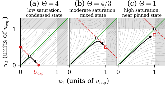
FIG. 3. The pinning saddle across \Theta . Phase portraits of the two-schema strength dynamics Eq. (24) in (u_1, u_2) , units of u_{\text{cap}} , at three budgets U_{\text{cap}} = Mu_{\text{cap}}/\Theta ( M = 2 throughout): the pinned (saddle) point (black-edged circle), at U_{\text{cap}}/2 , moves out along the stable manifold u_1 = u_2 (green) panel to panel as U_{\text{cap}} \rightarrow Mu_{\text{cap}} . The black curve is a trajectory from one seeded start (black dot, the same in all three panels), which grows along the stable manifold and then departs along the unstable one. (a) \Theta = 4 : the budget alone halts growth well inside u_{\text{cap}} , so the unstable manifold (red, condensation) runs to a genuinely reached bare condensate (filled circles). (b) \Theta = 4/3 : the ceiling is now reached first, arresting the same departure at u_{\text{cap}} (red square) before it reaches the excluded region u_1 > u_{\text{cap}} or u_2 > u_{\text{cap}} (shaded). (c) \Theta = 1 : capacity exactly meets demand ( M_{\text{cap}} = M ), so the saddle sits at u_1 = u_2 = u_{\text{cap}} and the trajectory is arrested (red square) just short of it. Panel sub-titles name the resulting state.
