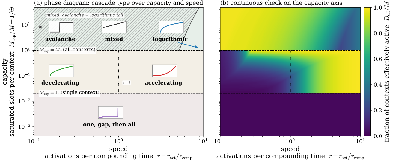
FIG. 4. Cascade types and repertoire size over replicator dynamics. Endogenous cascade regimes over the two coordinates that separate them. The horizontal axis ( speed ) is r = r_{\text{act}}/r_{\text{comp}} , the number of axes that activate per compounding time 1/r_{\text{comp}} , fixed by the dispersion of the seeded repertoire through Eq. (26). The vertical axis ( capacity ) is M_{\text{cap}}/M , the saturated slots per context, that is the fraction of the M candidate schemas the finite social capacity can sustain as live contexts ( M_{\text{cap}} = U_{\text{cap}}/u_{\text{cap}} ). (a) Phase diagram: where each cascade type sits in the plane. The capacity coordinate alone, \Theta = M/M_{\text{cap}} , splits it into three bands with sharp counting-threshold boundaries, the contexts the society can sustain being all M , a graded cluster of M_{\text{cap}} , or one. Inset sketches show the sequence of activations the transient sort passes through, set by r : avalanche to logarithmic in the thick band ( \Theta \leq 1 ), decelerating ( a > 1 ) to accelerating ( a < 1 ) across a = 1 in the middle band, and one onset, a gap, then all the rest in the thin band. The left-hand arrow marks r \rightarrow 0 , where the cascade is a pure avalanche. The random Marčenko–Pastur class (iv of Fig. 2) is absent because the loop selects endpoints, and an unstructured random spectrum is an initial condition rather than an endpoint (Sec. IV B). Within the thick band a saturated cluster coexists with a geometric tail (hatched) below the exact boundary r = M/L(\Theta) . The right-hand arrow runs from the logarithmic sketch past that boundary to a purely geometric spectrum, and the inset shows N(\beta) at a coexistence point—an early jump as the cluster ignites at once, then the tail’s gradual rise. (b) Continuous check on the capacity axis: the contexts effectively active , the participation ratio D_{\text{eff}} = (\sum_k \mu_k)^2 / \sum_k \mu_k^2 of the spectrum \{\mu_k = u_k\} , normalized by M , a continuous counterpart to the count M_{\text{cap}}/M on the vertical axis. It depends on how far the transient sort has progressed, hence on r , and falls below capacity wherever the sort is incomplete—bright on the accelerating side, darker on the decelerating side. The difference between the panels measures distance from the stationary endpoint. Exact boundaries, their mean-field status, the ceiling u_{\text{cap}} , and the held-fixed groups ( \alpha\langle\lambda\rangle/\kappa , \beta\mu_1/\gamma , M/d ) in Sec. IV B.
