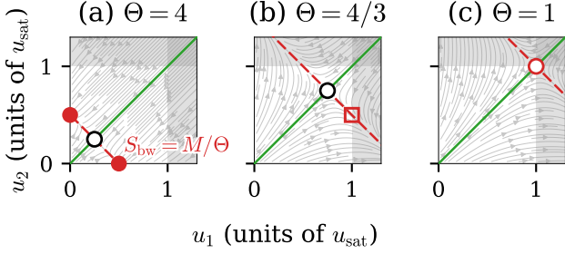
FIG. 4. The pinning saddle across \Theta . Phase portraits of the two-schema replicator Eq. (22) in (u_1, u_2) , units of u_{\text{sat}} , at three budgets S_{\text{bw}} ( M = 2 throughout): the pinned (saddle) point (black-edged circle), at S_{\text{bw}}/2 , climbs the stable manifold u_1 = u_2 (green) panel to panel as S_{\text{bw}} \rightarrow Mu_{\text{sat}} . (a) \Theta = 4 : the budget alone binds well inside u_{\text{sat}} , so the unstable manifold (red, condensation) runs to a genuinely reached bare condensate (filled circles). (b) \Theta = 4/3 : the ceiling now binds first, arresting the same flight at u_{\text{sat}} (red square) before it reaches the excluded region u_1 > u_{\text{sat}} or u_2 > u_{\text{sat}} (shaded). (c) \Theta = 1 : the saddle itself (now red-edged) sits exactly at u_1 = u_2 = u_{\text{sat}} , the boundary where capacity exactly meets demand ( M_{\text{cap}} = M ).
