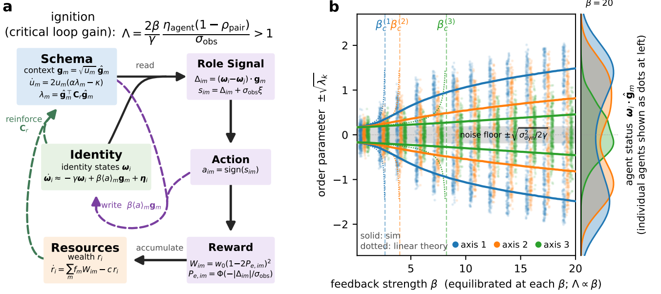
FIG. 1. The self-consistent schema–role–resource loop and its ignition. (a) Model schematic, separating the three persistent state variables (left: context schemas \mathbf{g}_m = \sqrt{u_m} \hat{\mathbf{g}}_m , of which only the strength u_m evolves; identities \boldsymbol{\omega}_i ; and agent resources r_i ) from the fast per-encounter signal chain (right: signal s_{im} , action a_{im} , reward W_{im} ). Solid arrows are the feed-forward read-out: schema and identity form the status signal (the schema \mathbf{g}_m is the axis along which the status difference \Delta_{im} is read), the policy thresholds it into an action, and the resulting coordination reward accumulates as resources. Dashed arrows are the slow state updates that close the loop: resources reweight identities to reinforce schemas through the resource-weighted covariance \mathbf{C}_r , and actions are inscribed back into identities along the same axis (the write \beta(a)_m \mathbf{g}_m ). The single direction \mathbf{g}_m thus serves as both read and write axis, making Sewell’s schema–role duality a fixed-point loop. Each encounter is the information-engine cycle—read a noisy status, decide, earn a coordination reward (the engine’s analog of extracted work)—and the engine ignites when the loop gain \Lambda > 1 (top). (b) Three sequential bifurcations (order parameter vs. coupling) over the \beta sweep ( N = 2500 , d = M = 3 , hierarchical fixed context repertoire, random pairing; Methods). Points are individual agent statuses \boldsymbol{\omega}_i \cdot \hat{\mathbf{g}}_m along the three schema axes (snapshots of the agent cloud at each \beta ); solid curves are the order parameter \pm \sqrt{\lambda_k} , the two branches of a pitchfork on each axis, with \lambda_k the k -th eigenvalue of the population covariance \mathbf{C} . Below its critical coupling an axis is unimodal within the noise band \pm \sqrt{\sigma_{\text{dyn}}^2/2\gamma} ; above it (dashed lines) it splits into two role modes—the complementary leader/follower assignments of the anti-coordination game—which separate further with \beta . Dotted curves are the linear mean-field theory \lambda_k = \sigma_{\text{dyn}}^2/2(\gamma - \beta(1 - \rho_{\text{pair}})\mu_k) ( \mu_k = 2\pi'(0)u_k ), diverging at \beta_c^{(k)} = \gamma/[(1 - \rho_{\text{pair}})\mu_k] (random pairing, \rho_{\text{pair}} = 0 ) while the quartic confinement saturates the simulated branch—the visible cascade signature. Axis 1 splits first, then axis 2, then axis 3. The right strip shows the status distribution at \beta = 20 on the shared axis: axis 1 fully bimodal, axis 3 only marginally. The left axis reads the branches as the order parameter, the right axis the agents’ status; both are the same role projection. Schemas are held fixed here to display the cascade cleanly; the full loop selects this ordering endogenously through resource feedback (Fig. 3).
