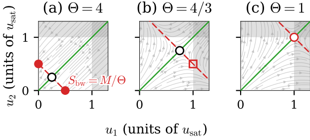
FIG. 4. The pinning saddle across \Theta . Phase portraits of the two-schema strength dynamics Eq. (22) in (u_1, u_2) , units of u_{\text{sat}} , at three budgets S_{\text{bw}} ( M = 2 throughout): the pinned (saddle) point (black-edged circle), at S_{\text{bw}}/2 , climbs the stable manifold u_1 = u_2 (green) panel to panel as S_{\text{bw}} \rightarrow Mu_{\text{sat}} . (a) \Theta = 4 : the budget alone binds well inside u_{\text{sat}} , so the unstable manifold (red, condensation) runs to a genuinely reached bare condensate (filled circles). (b) \Theta = 4/3 : the ceiling now binds first, arresting the same flight at u_{\text{sat}} (red square) before it reaches the excluded region u_1 > u_{\text{sat}} or u_2 > u_{\text{sat}} (shaded). (c) \Theta = 1 : the saddle itself (now red-edged) sits exactly at u_1 = u_2 = u_{\text{sat}} , the boundary where capacity exactly meets demand ( M_{\text{cap}} = M ).
