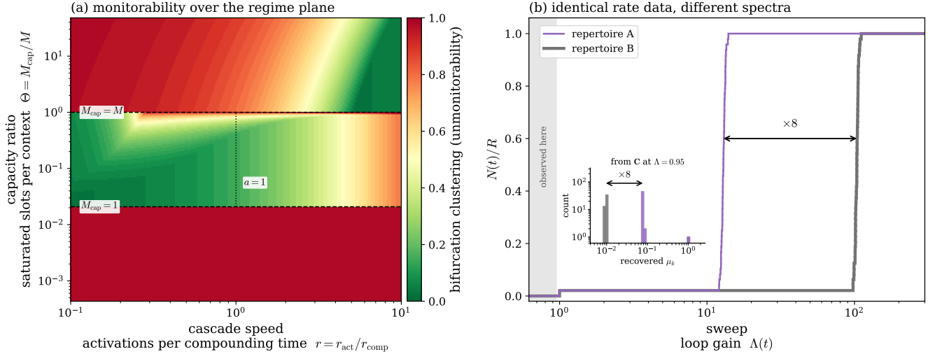
FIG. 5. Monitoring the cascade. (a) Monitorability over the (\Theta, r) plane: the clustering of bifurcation onsets (colour; the maximal share arriving within \Delta \ln \Lambda = 0.15 , hence unmonitorability), red where onsets cluster into a single burst (avalanche, spiked) and green where they resolve into a sequence (logarithmic, decelerating). The \Theta boundaries are sharp, the r dependence a smooth crossover. Regime layout as in Fig. 4. (b) The measurement term, under a linear sweep of the loop gain \Lambda(t) . Two repertoires whose counting functions coincide over the whole plotted range: each activates one axis at \Lambda = 1 and then stays quiescent. In repertoire A the remaining R - 1 modes sit just below threshold and avalanche at \Lambda = 13 ; in repertoire B the same modes sit far below and do not activate until \Lambda = 104 . The two spectra differ only below 1/\Lambda , which the bifurcation rate never samples, so rate extrapolation cannot separate them. Inset: the gain spectrum recovered from the subcritical covariance \mathbf{C} = \frac{\sigma_\omega^2}{2\gamma} (\mathbf{I}_{d \times d} - \mathbf{\Lambda})^{-1} at \Lambda = 0.95 , before either has bifurcated. The two recovered bulks are separated by the same factor of 8 that separates the two rises, since an onset sits at 1/\mu . The paired arrows mark it. The inversion amplifies a 7% difference in covariance eigenvalues into that factor, so the number of agents sampled sets the practical limit (Sec. V).
