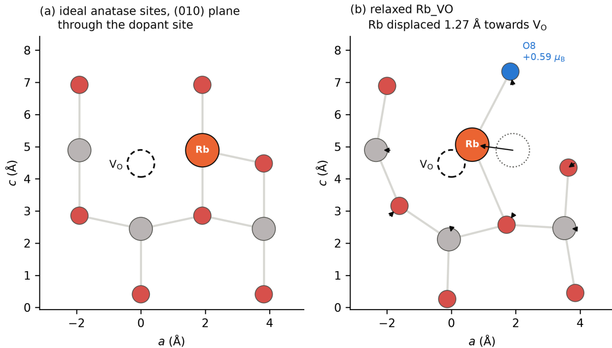
Figure 1. The (010) atomic plane containing the dopant site and the oxygen vacancy. (a) Ideal anatase positions built with the lattice parameters of this work ( a = 7.63632 Å, c = 9.77900 Å, u = 0.208 ), with the dopant on the substituted Ti site and the vacant oxygen site marked by a dashed circle. (b) The same plane in the relaxed Rb_VO cell (PBE+U, U(\text{Ti-3d}) = 3.5 eV, \Gamma -only), from the final coordinates of the production relaxation. Arrows give the displacement (where larger than 0.2 Å) of each in-plane atom from its ideal site after removal of the mean displacement; the dotted circle marks the ideal Rb site. The oxygen drawn in blue (O8) carries the largest Löwdin spin polarisation (+0.59 μ B ; Section 3.6, Figure S1). Grey: Ti; red: O; orange: Rb. Only atoms in the plane are drawn, so each Ti shows fewer than six bonds. Plotted from the pw.x output by figures/make_fig1_structures.py.
