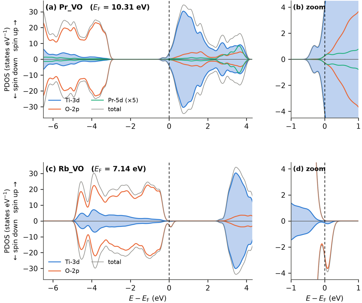
Figure 4. Spin-resolved projected densities of states of (a) Pr_VO and (c) Rb_VO , with (b, d) the region within \pm 1 eV of E_F , from 2 \times 2 \times 2 non-self-consistent calculations on the relaxed cells (PBE+U, U(\text{Ti-3d}) = 3.5 eV; tetrahedron occupations; Gaussian broadening 0.01 Ry). Spin up is plotted upwards and spin down downwards; energies are relative to each cell's Fermi level (10.31 and 7.14 eV). Filled blue: Ti-3d summed over 15 Ti; orange: O-2p summed over 31 O; green: Pr-5d multiplied by 5; grey: total. The Rb dataset has no d projector, so no dopant-d channel exists for Rb_VO . In (b) the occupied conduction-band states have equal weight in the two spin channels, as the m = 0 density implies (95 % Ti-3d; the broadened DOS holds 0.70 states per channel between -0.6 eV and E_F for 0.5 electrons). In (d) the empty band just above E_F (0.04–0.13 eV in the eigenvalues) appears in the spin-down channel only (93 % O-2p; broadened weight 0.79 states between E_F and +0.6 eV). Plotted without smoothing from the summed projwfc.x output by figures/make_pdos_figures.py .
