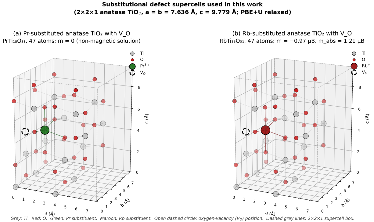
Figure 1. Relaxed 2 \times 2 \times 1 anatase supercells with one substitutional dopant and one oxygen vacancy (PBE+U, U(Ti-3d) = 3.5 eV, \Gamma -only). (a) Pr Ti + V_O (PrTi 15 O 31 , 47 atoms), non-magnetic solution ( m = 0 ). (b) Rb Ti + V_O (RbTi 15 O 31 , 47 atoms), m = -0.97 \mu_B , m_{abs} = 1.21 \mu_B . Grey: Ti; red: O; green: Pr; maroon: Rb; dashed circle: vacancy position; dashed box: supercell. [AUTHOR ACTION: the panel subtitles of the interim artwork were patched to match this caption; regenerate the figure from the relaxed coordinates and add the vacancy atom index and dopant- V_O distance to each panel.]
