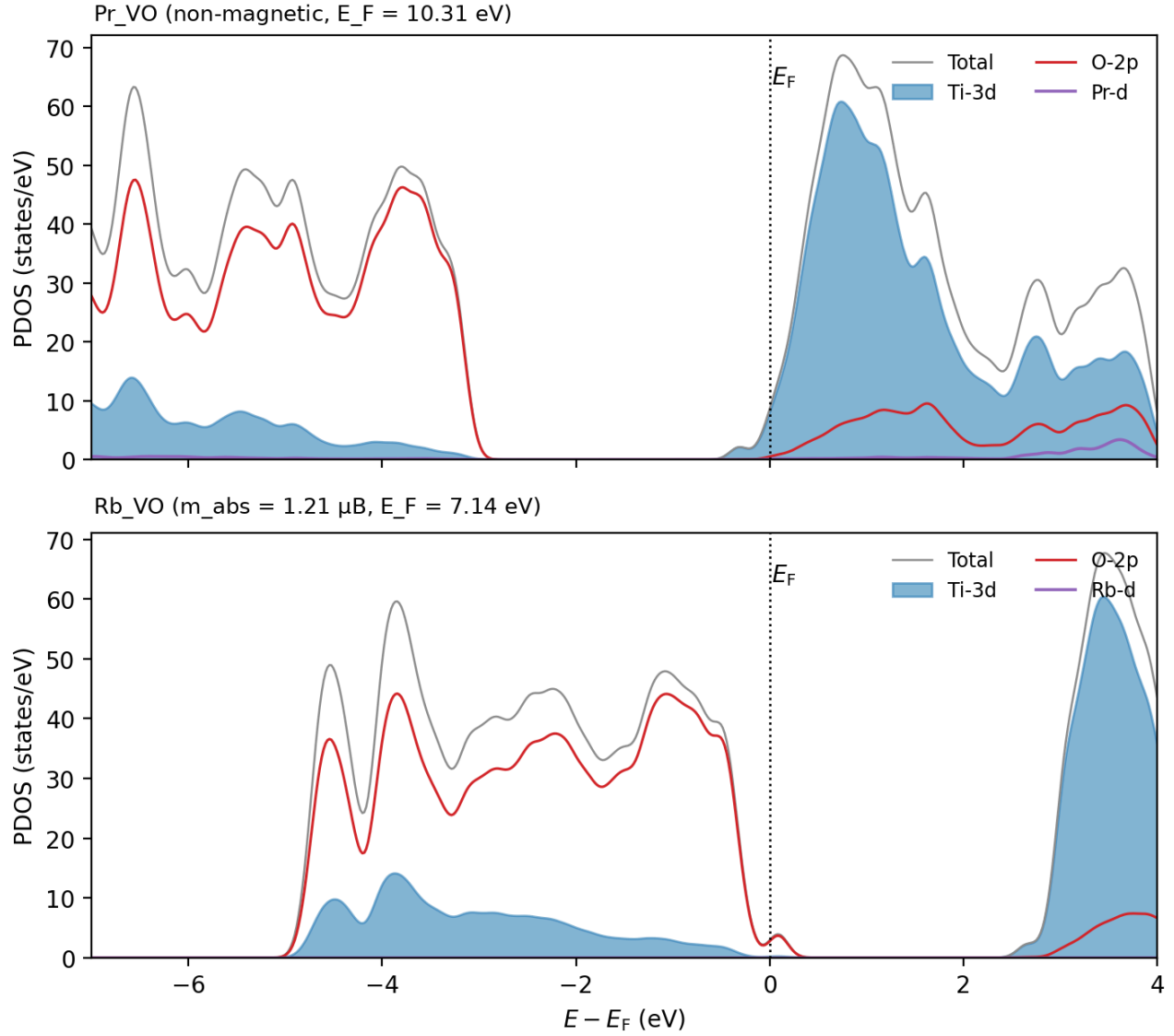
Figure S2. Projected density of states of Pr_VO (top) and Rb_VO (bottom) without spin decomposition. Filled: Ti-3d; red: O-2p; purple: dopant d; grey: total.
