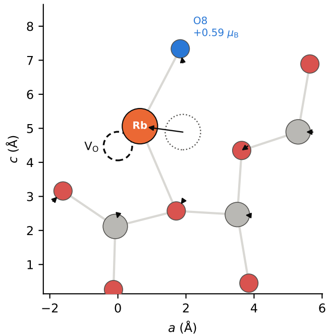
(b) relaxed Rb_VO Rb displaced 1.27 Å toward V_O
