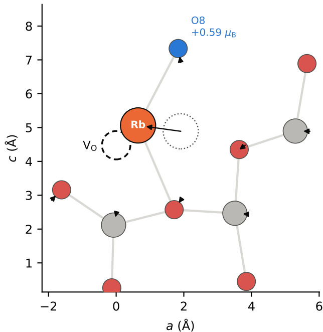
(b) relaxed Rb_VO Rb displaced 1.27 Å toward V_o
