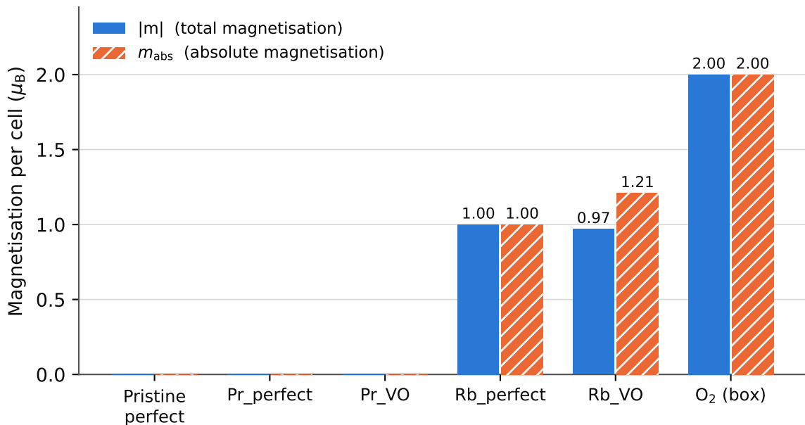
Converged magnetisation, single-U(Ti-3d) PBE+U relaxations
