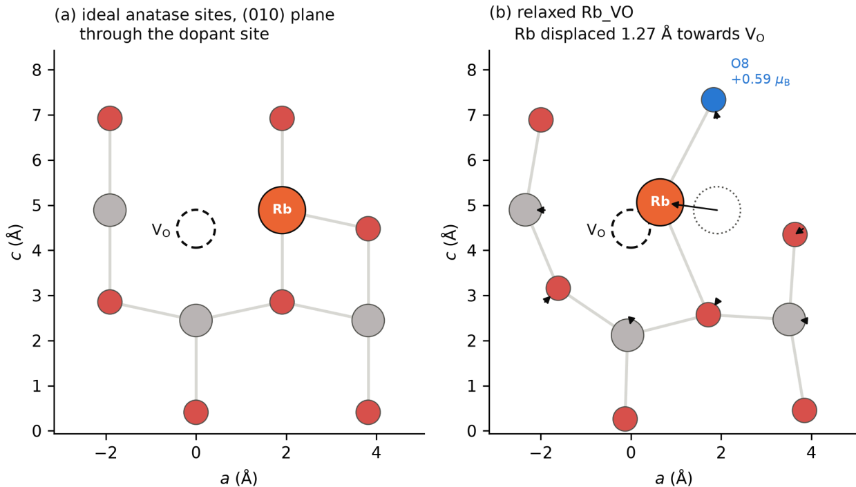
Figure 1. The (010) atomic plane containing the dopant site and the oxygen vacancy. (a) Ideal anatase positions built with the lattice parameters of this work ( a = 7.63632 \text{ Å} , c = 9.77900 \text{ Å} , u = 0.208 ), with the dopant on the substituted Ti site and the vacant oxygen site marked by a dashed circle. (b) The same plane in the relaxed Rb_VO cell (PBE+U, U(\text{Ti-3d}) = 3.5 \text{ eV} , \Gamma -only), from the final coordinates of the production relaxation. Arrows give the displacement (where larger than 0.2 \text{ Å} ) of each in-plane atom from its ideal site after removal of the mean displacement; the dotted circle marks the ideal Rb site. The oxygen drawn in blue (O8) carries the largest Löwdin spin polarisation ( +0.59 \mu_B ; Section 3.6, Figure S1). Grey: Ti; red: O; orange: Rb. Only atoms in the plane are drawn, so each Ti shows fewer than six bonds. Plotted from the pw.x output by figures/make_fig1_structures.py.
