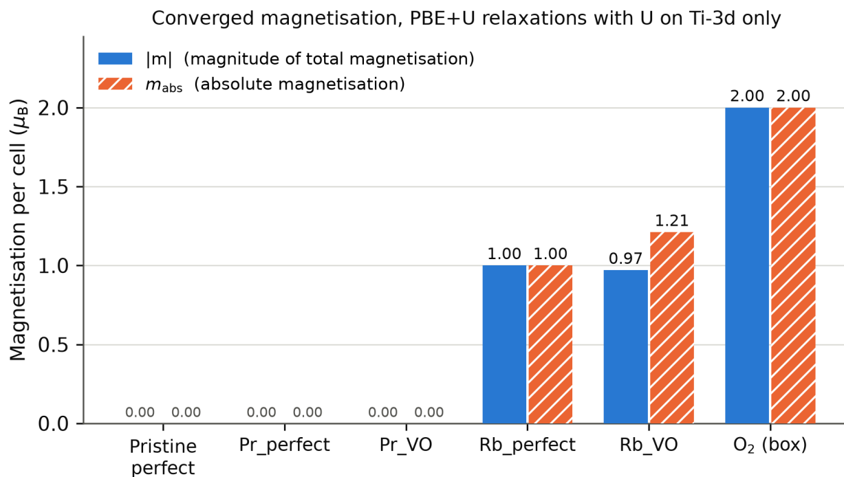
Figure 3. Magnitude of the total magnetisation ( |m| ) and absolute magnetisation ( m_{abs} ) of the production cells and of the O 2 reference (PBE+U relaxations with U on Ti-3d only). The Pr cells and the pristine cell converge to non-magnetic solutions; both Rb cells carry one unpaired spin, and Rb_VO shows m_{abs} > |m| .
