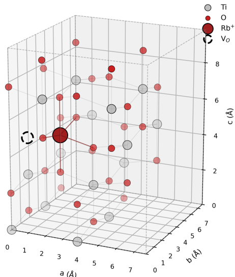
(b) Rb-substituted anatase TiO 2 with V_O RbTi 15 O 31 , 47 atoms; m = -0.97 μB, m_{\text{abs}} = 1.21 μB
