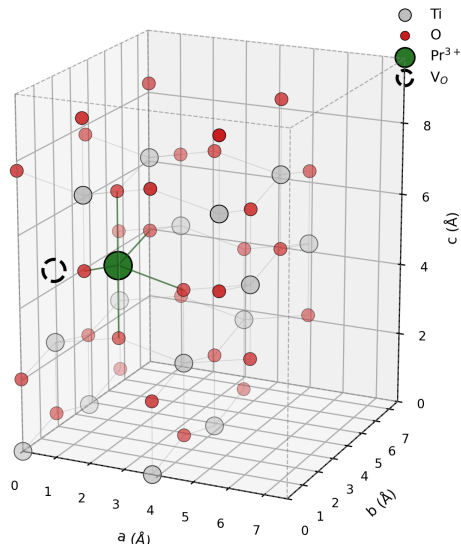
(a) Pr-substituted anatase TiO 2 with V_O PrTi 15 O 31 , 47 atoms; m = 0 (non-magnetic solution)
