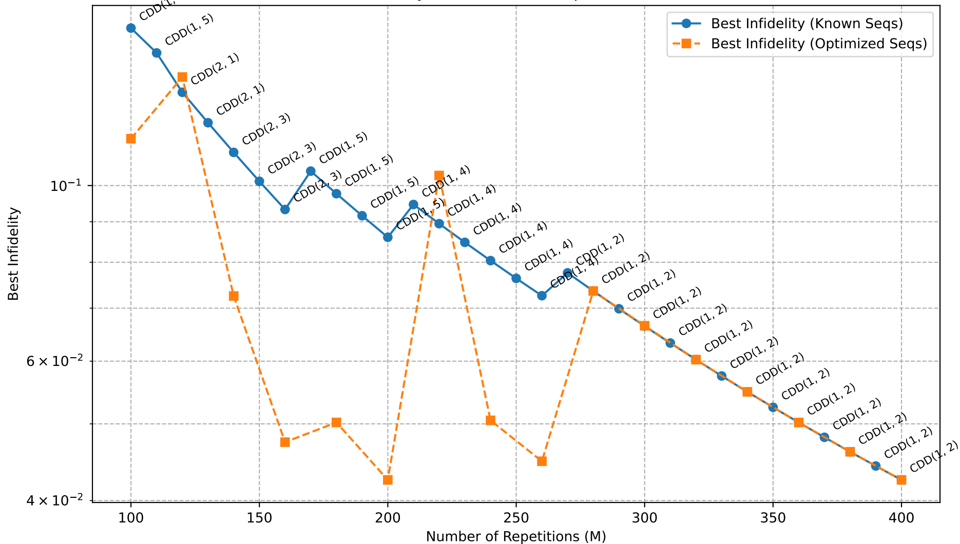
Infidelity vs. Number of Repetitions (M)
