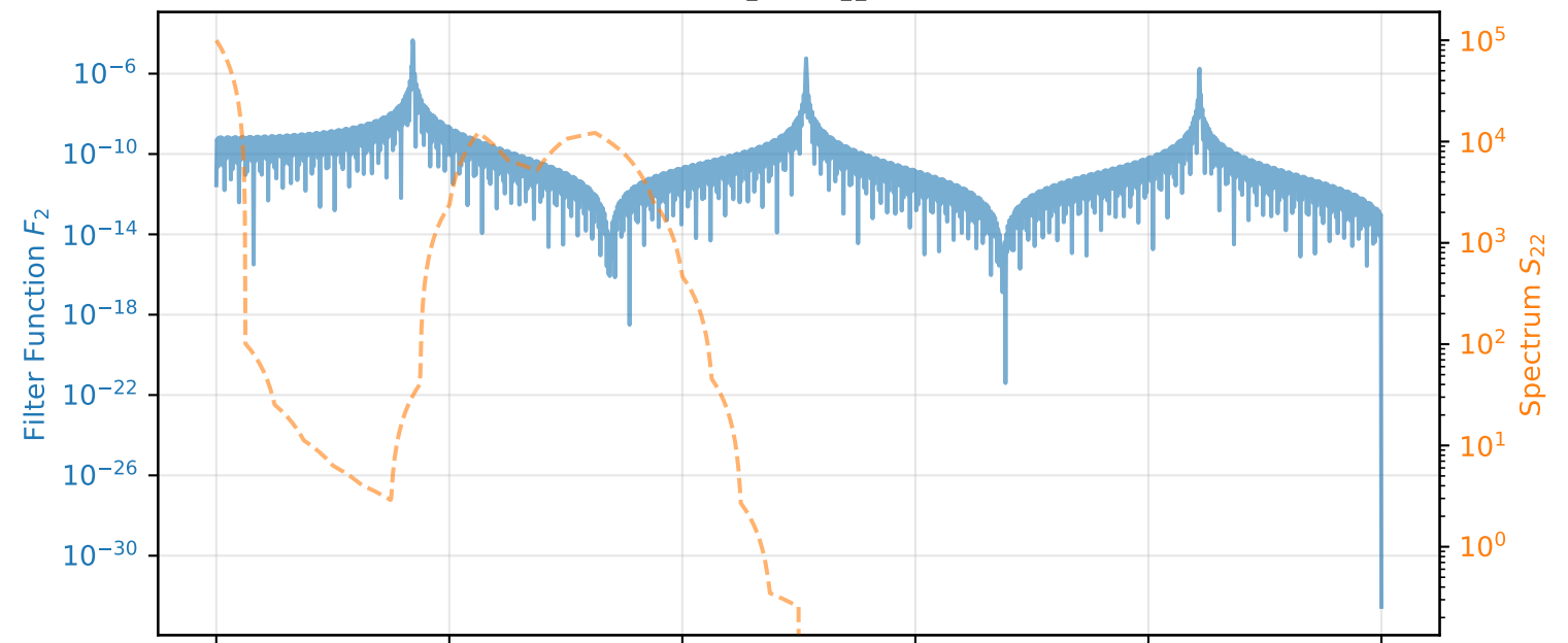
Best Optimized Sequence F_2 vs S_{22}
