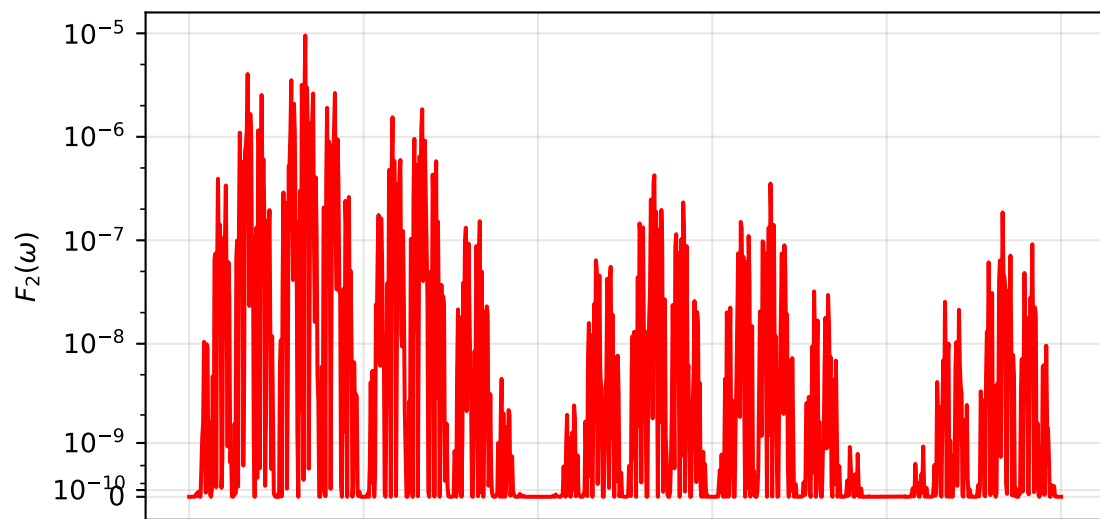
Qubit 2 Filter Function ( F_2 )
