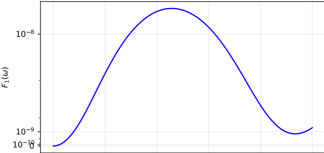
Best Optimized Sequence Qubit 1 Filter Function ( F_1 )
