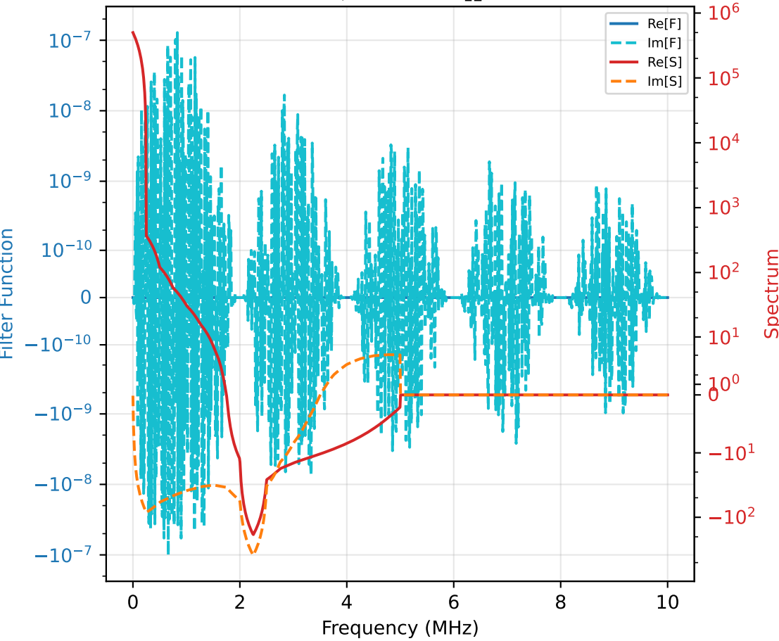
S_{1,12} and F_1 F_{12}^*
