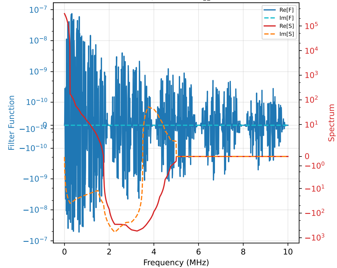
S_{2,12} and F_2 F_{12}^*
