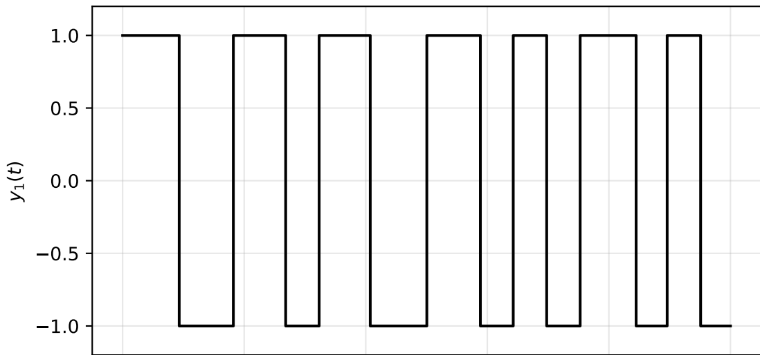
Best Optimized Sequence Qubit 1 Switching Function ( y_1 )
