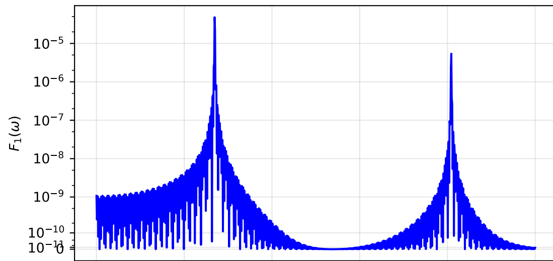
Best Optimized Sequence Qubit 1 Filter Function ( F_1 )
