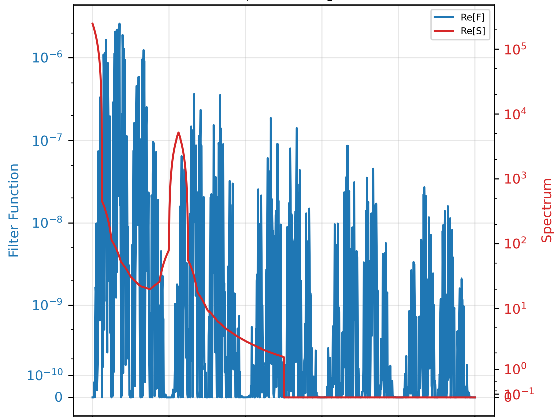
S_{1,1} and F_1 F_1^*
