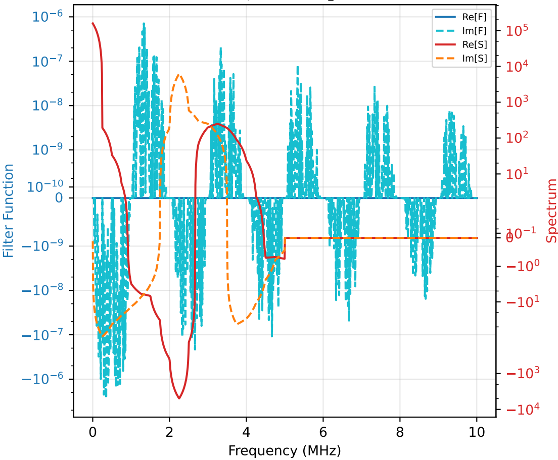
S_{1,2} and F_1 F_2^*
