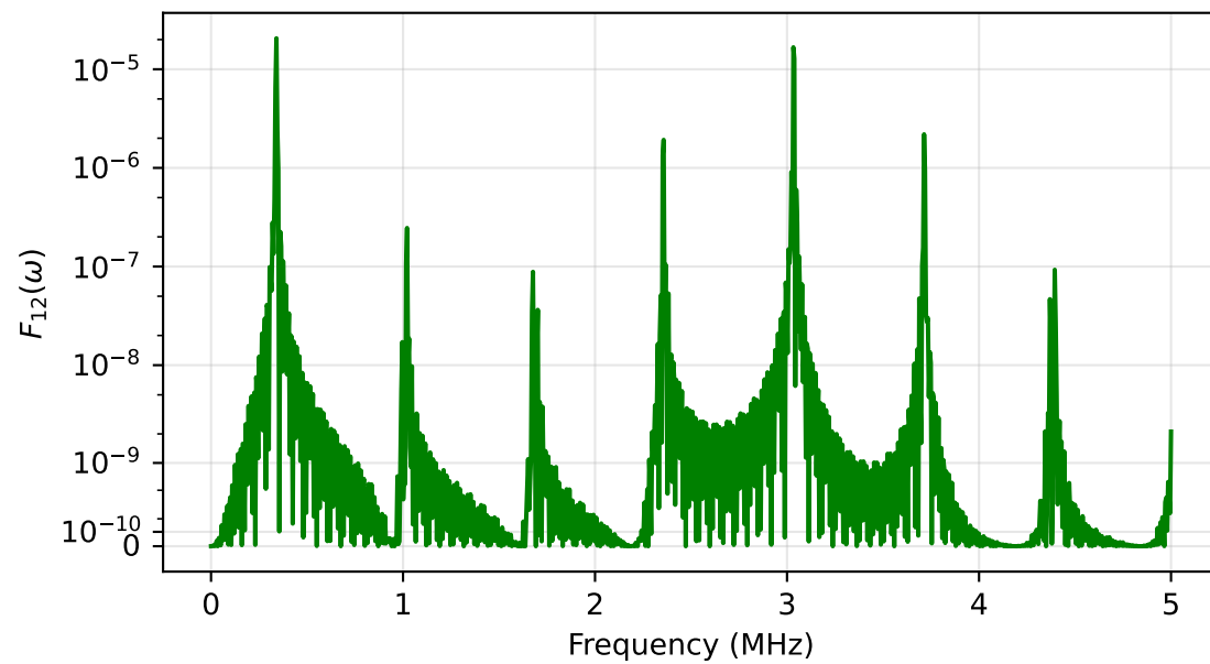
Interaction Filter Function ( F_{12} )
