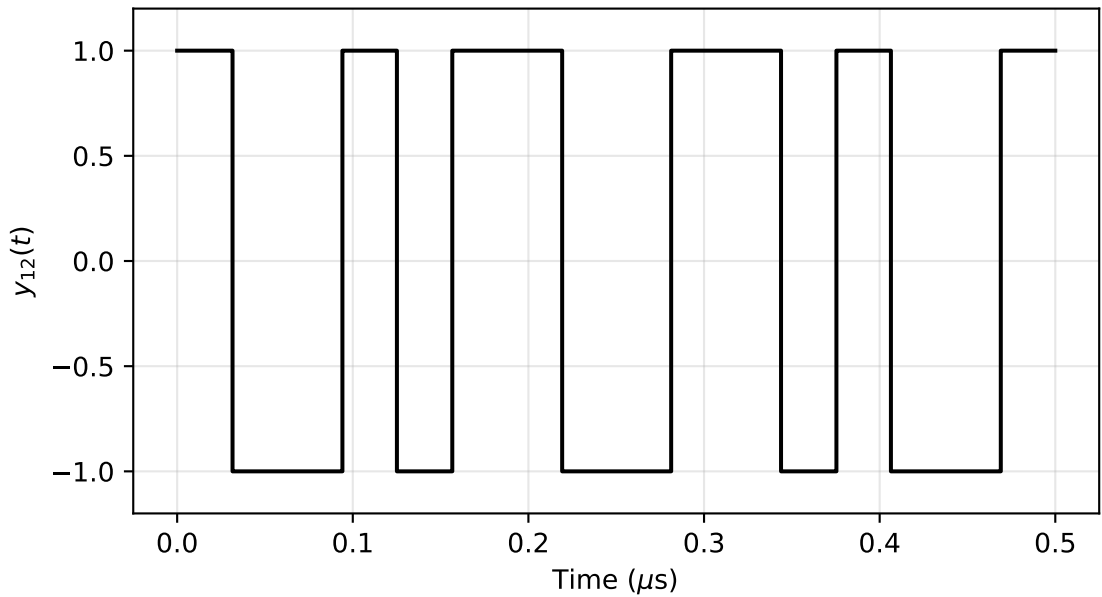
Interaction Switching Function ( y_{12} )
