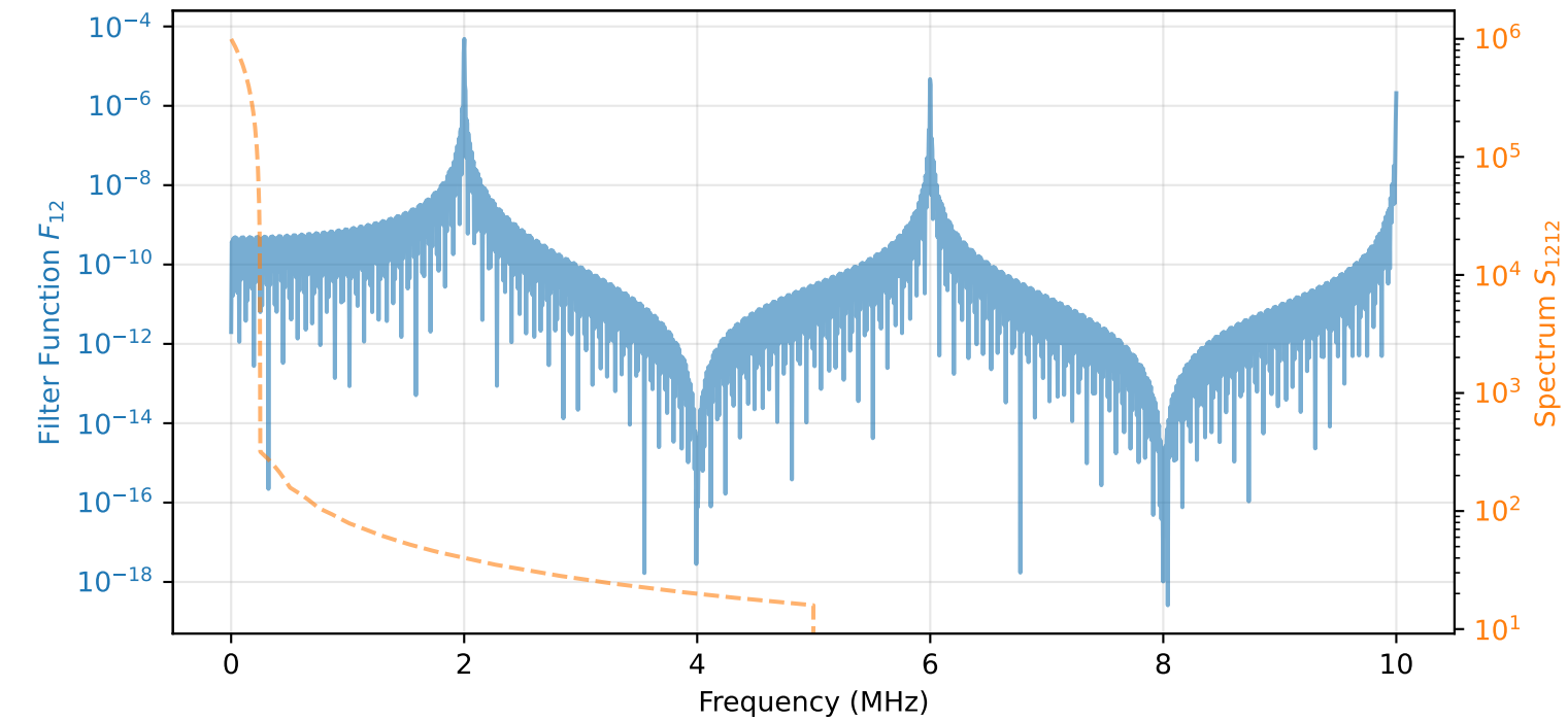
Best Known Sequence F_{12} vs S_{1212}
