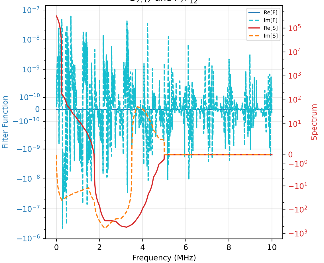
S_{2,12} and F_2 F_{12}^*
