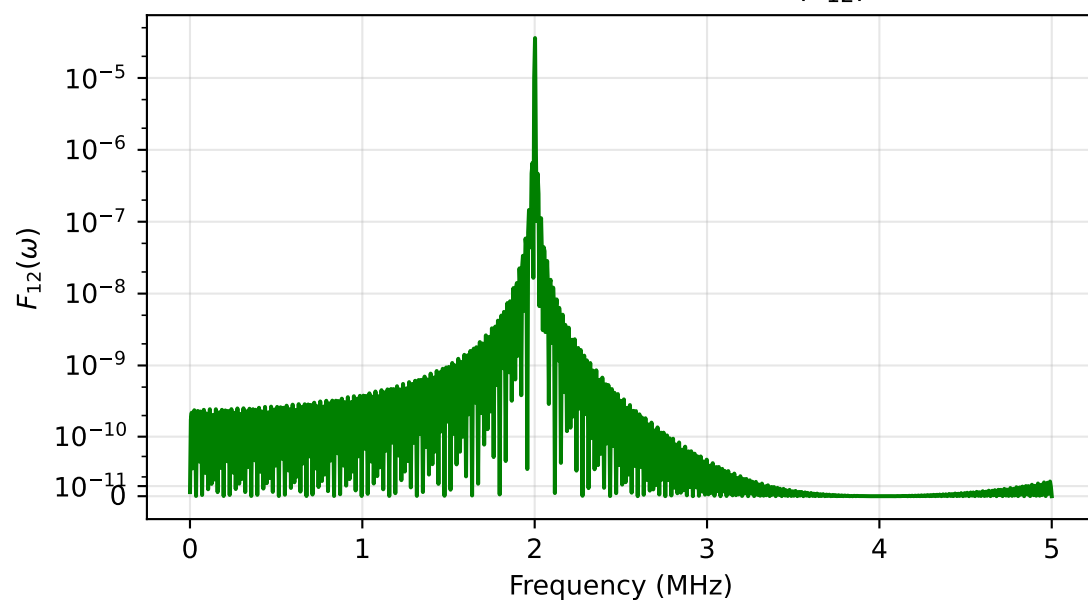
Interaction Filter Function ( F_{12} )
