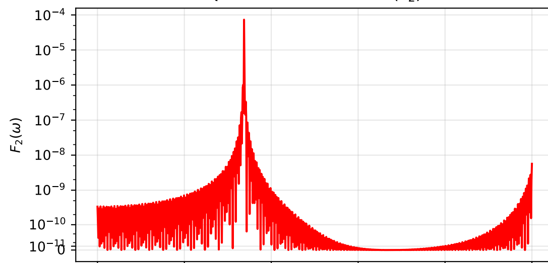
Qubit 2 Filter Function ( F_2 )
