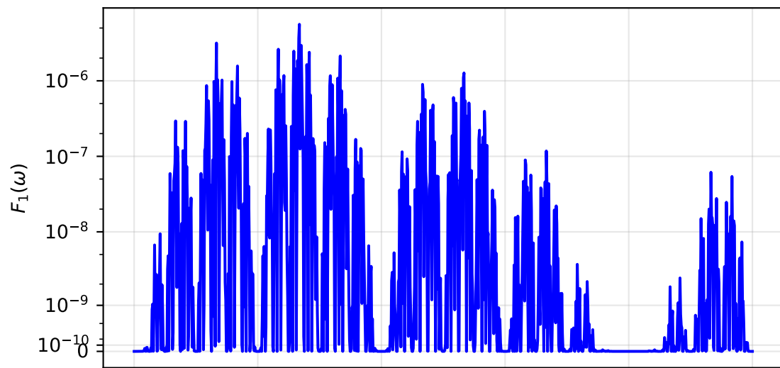
Best Known Sequence Qubit 1 Filter Function ( F_1 )
