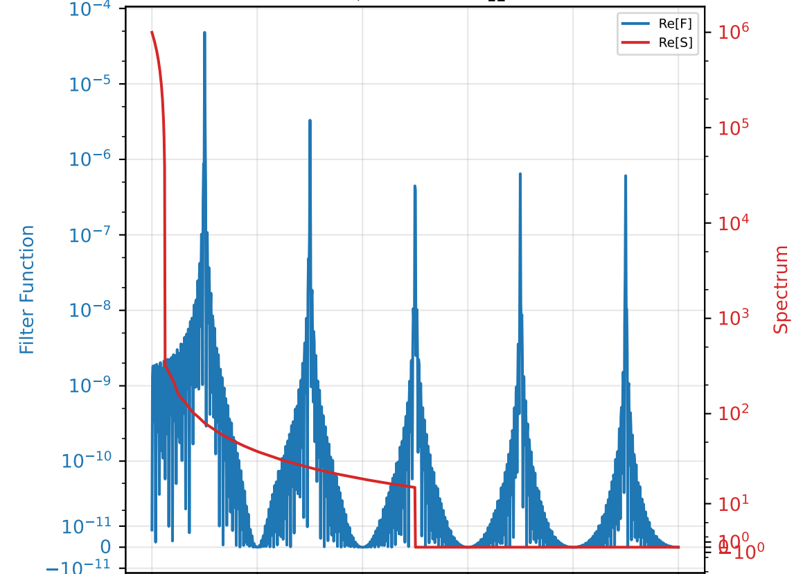
S_{12,12} and F_{12} F_{12}^*
