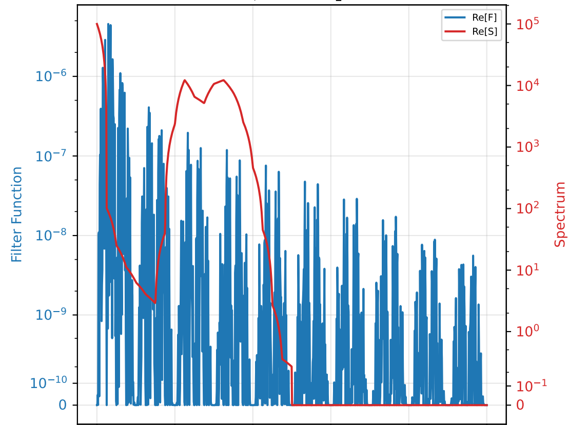
S_{2,2} and F_2 F_2^*
