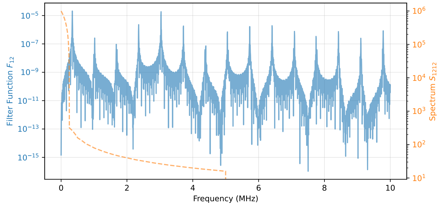
Best Optimized Sequence F_{12} vs S_{1212}
