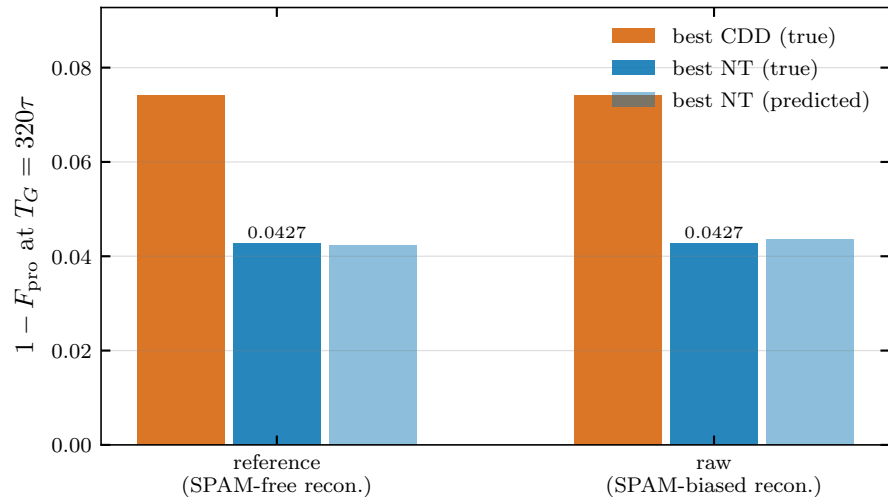
(d) idle: gates designed on SPAM-biased vs unbiased spectra
