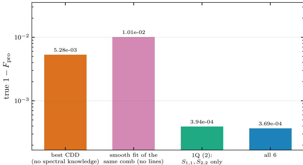
entangling (CZ): blind NT gate vs spectral knowledge given to the optimizer ( T_G = 320\tau )
