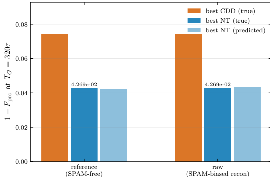
Ask 3: gates from biased vs unbiased spectra
