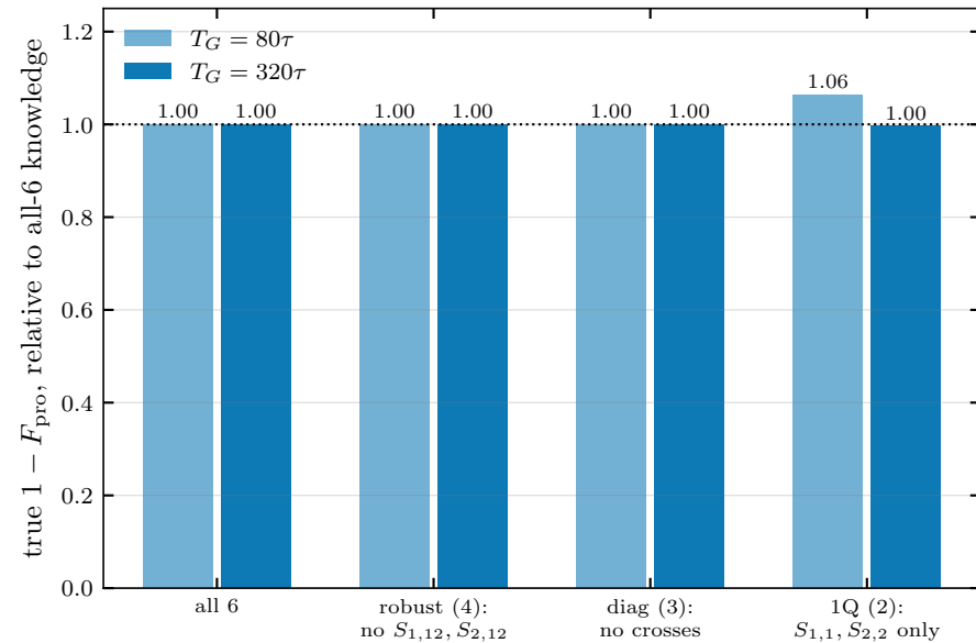
Ask 2: blind NT gate vs spectral knowledge
